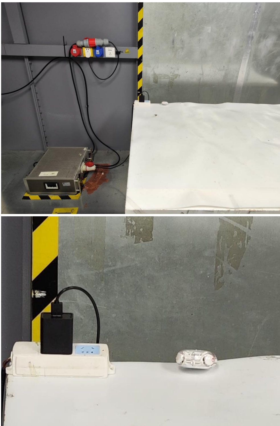
Photo of Conducted Emission test
