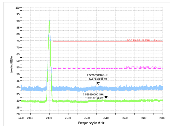
Test Mode: \pi/4 DQPSK-High Hopping-off
