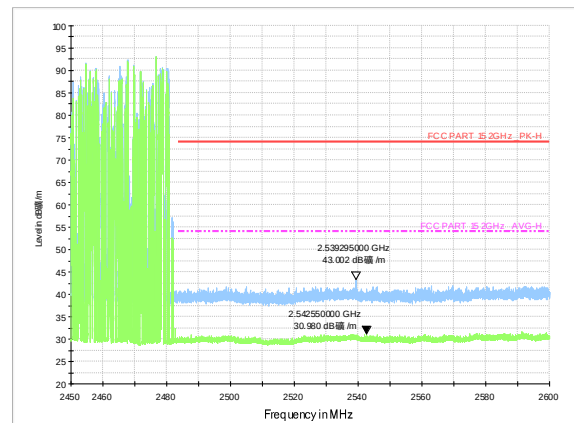
Test Mode: \pi/4 DQPSK-High Hopping-on
