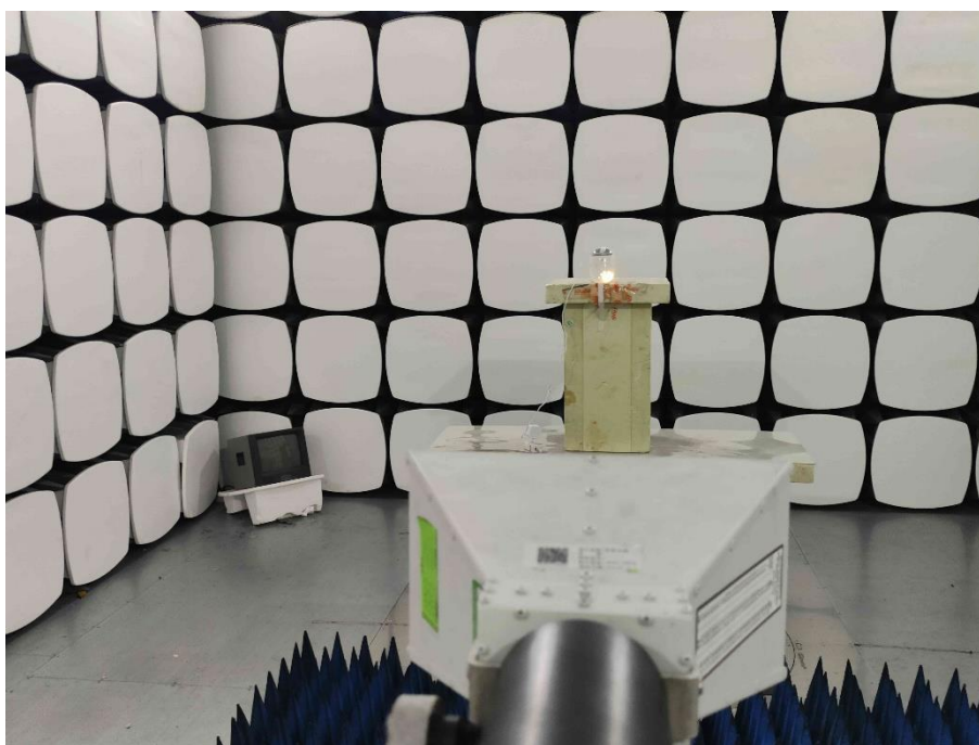
Radiated Emission test view (Frequency from Above 1GHz)
