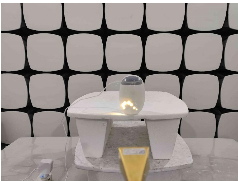
Radiated Emission test view (Frequency from 60GHz to 90GHz)
