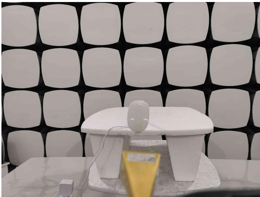
Radiated Emission test view (Frequency from 60GHz to 90GHz)
