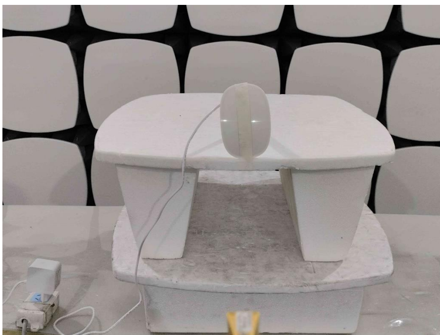
Radiated Emission test view (Frequency from 140GHz to 200GHz)
