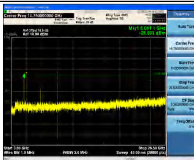
Band7-15MHz-16QAM-20825-1RB#0-Range5:3000~26500MHz
