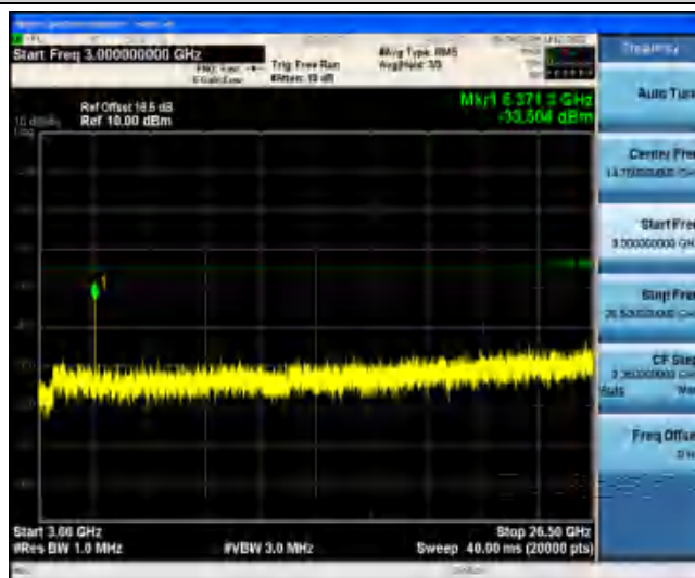
Band41-5MHz-16QAM-41565-1RB#0-Range5:3000~26500MHz
