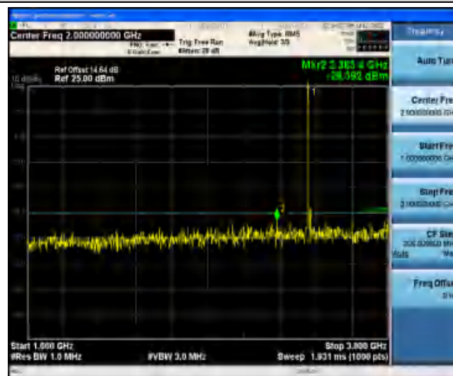
Band7-15MHz-16QAM-21375-1RB#0-Range4:1000~3000MHz
