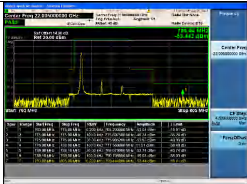
Band13_10MHz_QPSK_23230_1RB#0
