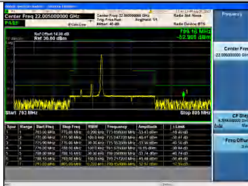
Band13_5MHz_16QAM_23205_1RB#24
