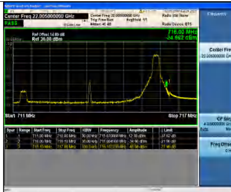
Band17_5MHz_16QAM_23825_1RB#24
