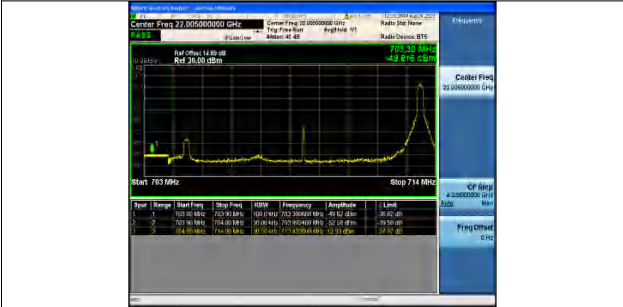
Band17_10MHz_QPSK_23780_50RB#0
