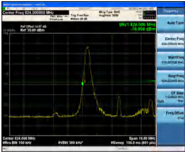
Band5-5MHz-16QAM-20425-1RB#24
