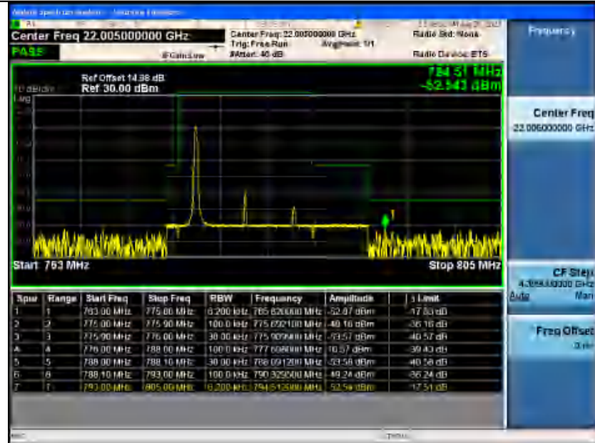
Band13_10MHz_16QAM_23230_1RB#0
