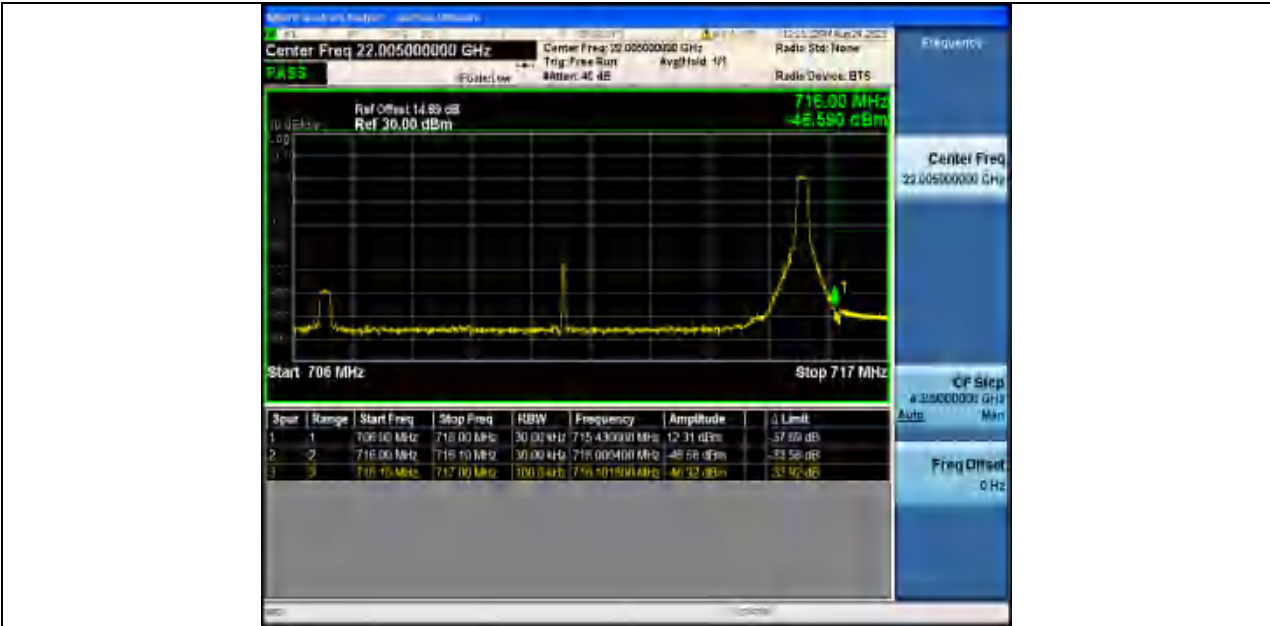
Band17_10MHz_16QAM_23800_1RB#49
