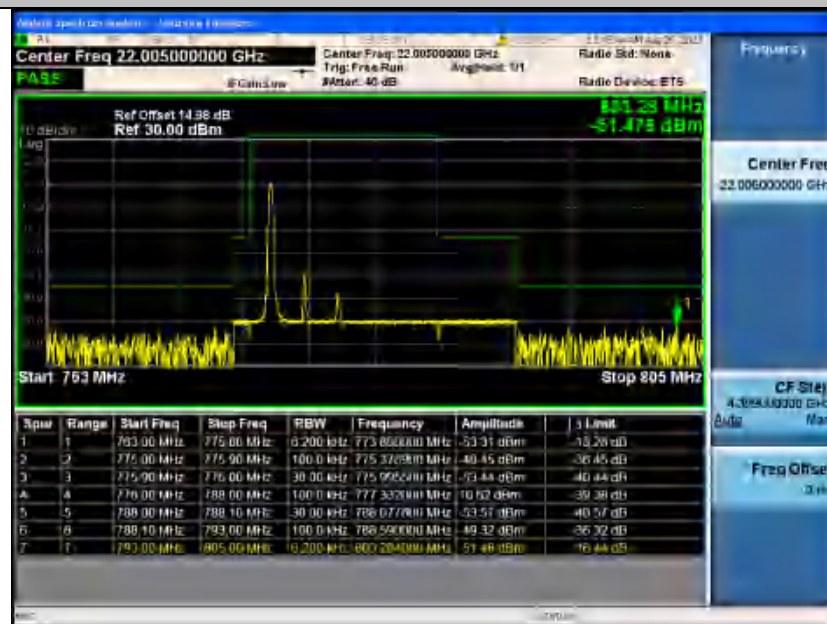
Band13_5MHz_16QAM_23205_1RB#0
