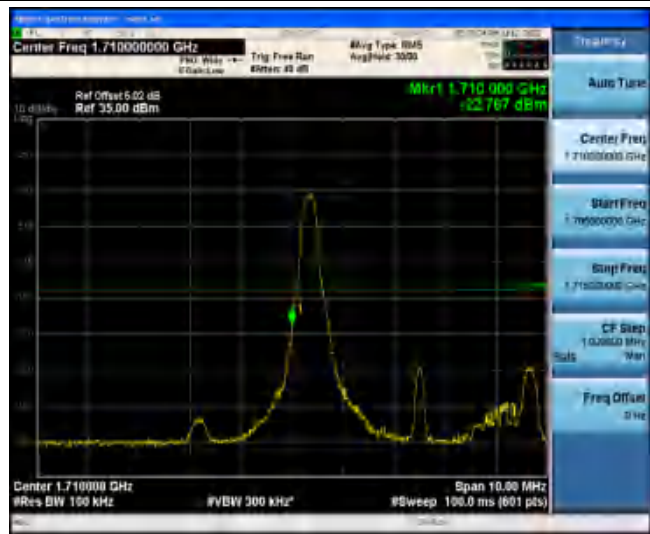
Band4-5MHz-16QAM-19975-1RB#24
