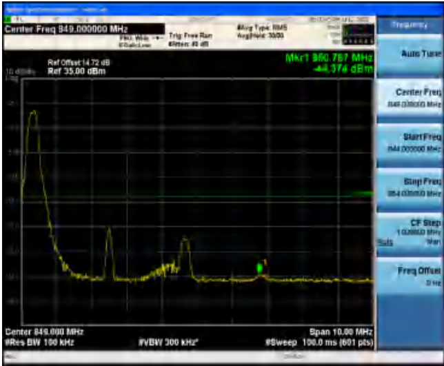
Band5-5MHz-16QAM-20625-1RB#24
