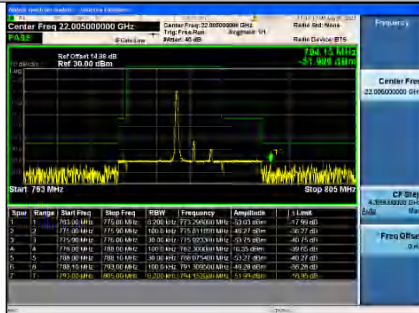
Band13_5MHz_16QAM_23255_1RB#0
