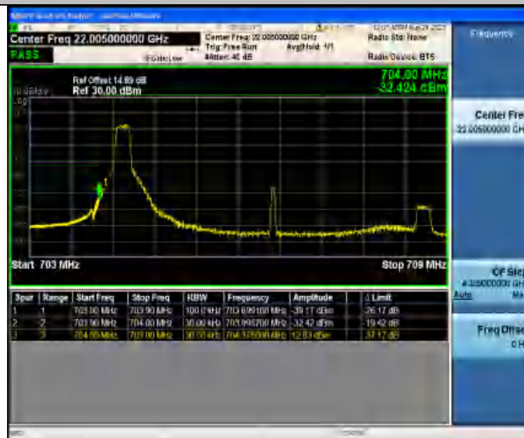
Band17_5MHz_QPSK_23755_1RB#24
