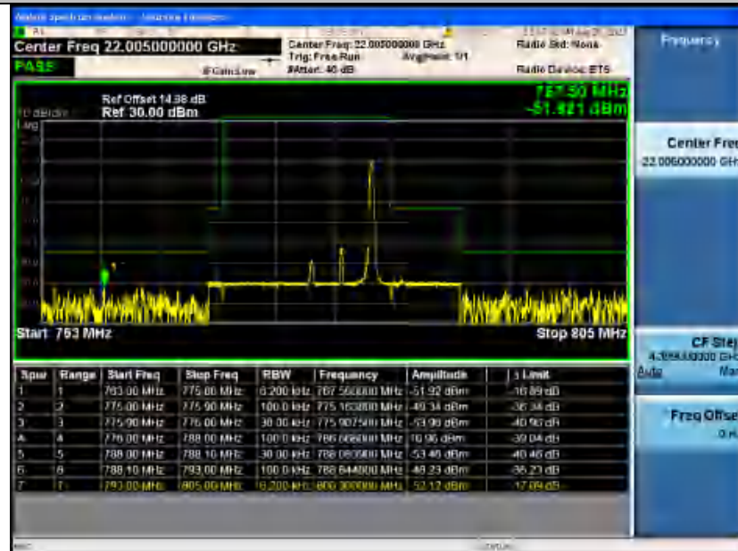
Band13_5MHz_16QAM_23255_1RB#24
