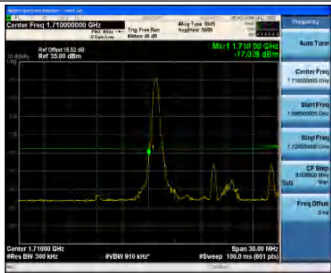
Band4-15MHz-QPSK-20025-1RB#74
