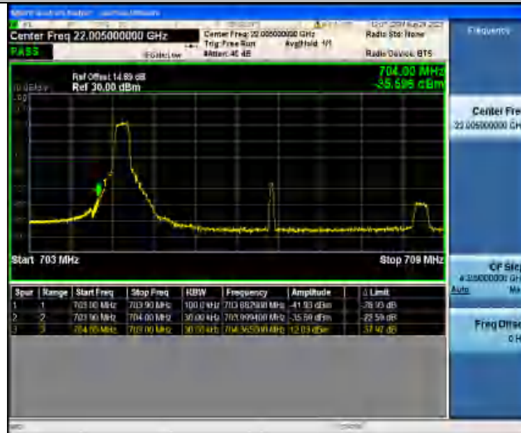
Band17_5MHz_16QAM_23755_1RB#0
