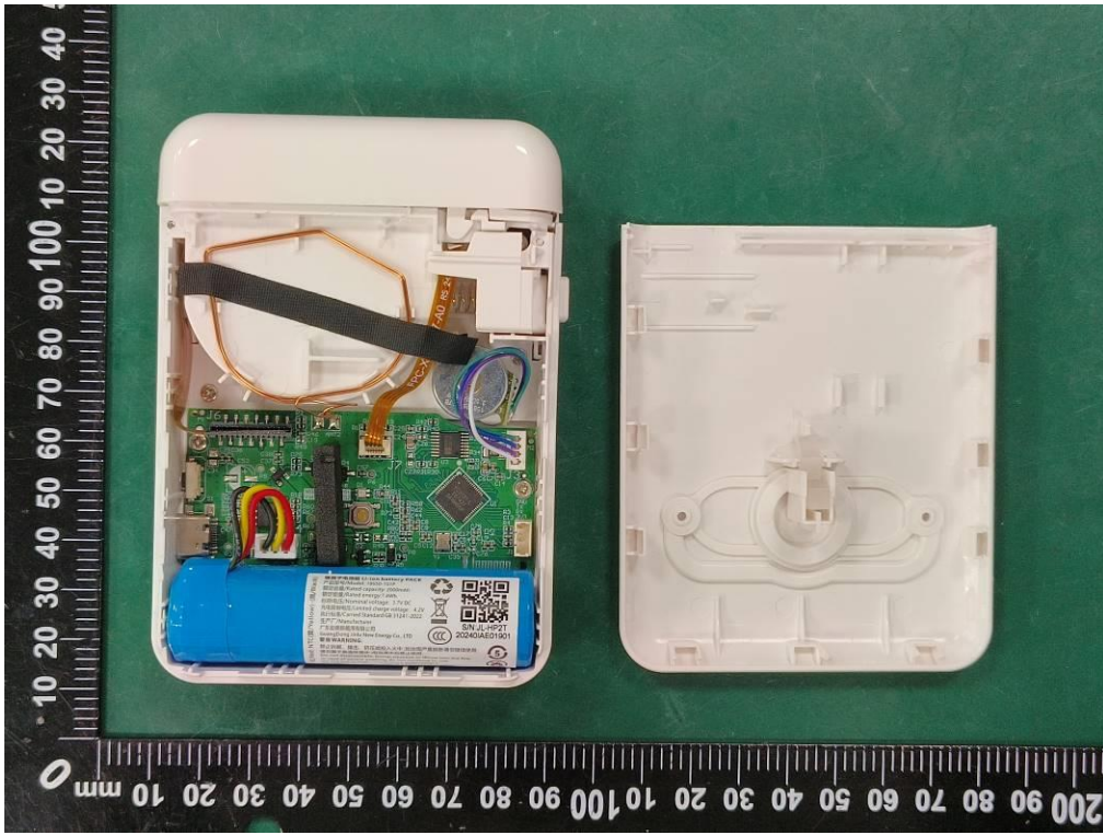
Internal Photo FCC ID: 2BCBZ-X1
