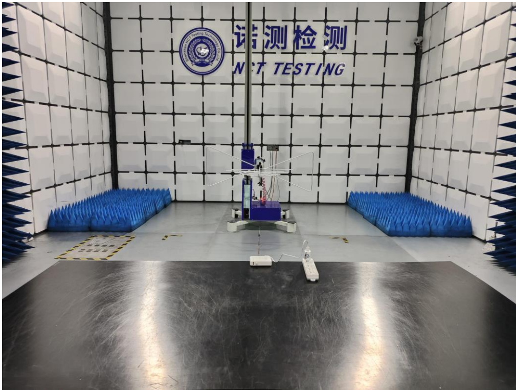
Setup Photo FCC ID: 2BCBZ-X1
