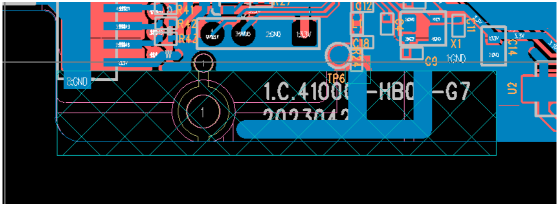
Antenna electronic spec
