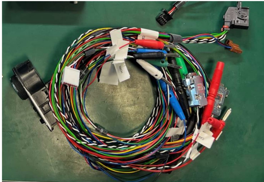
Cable harness
