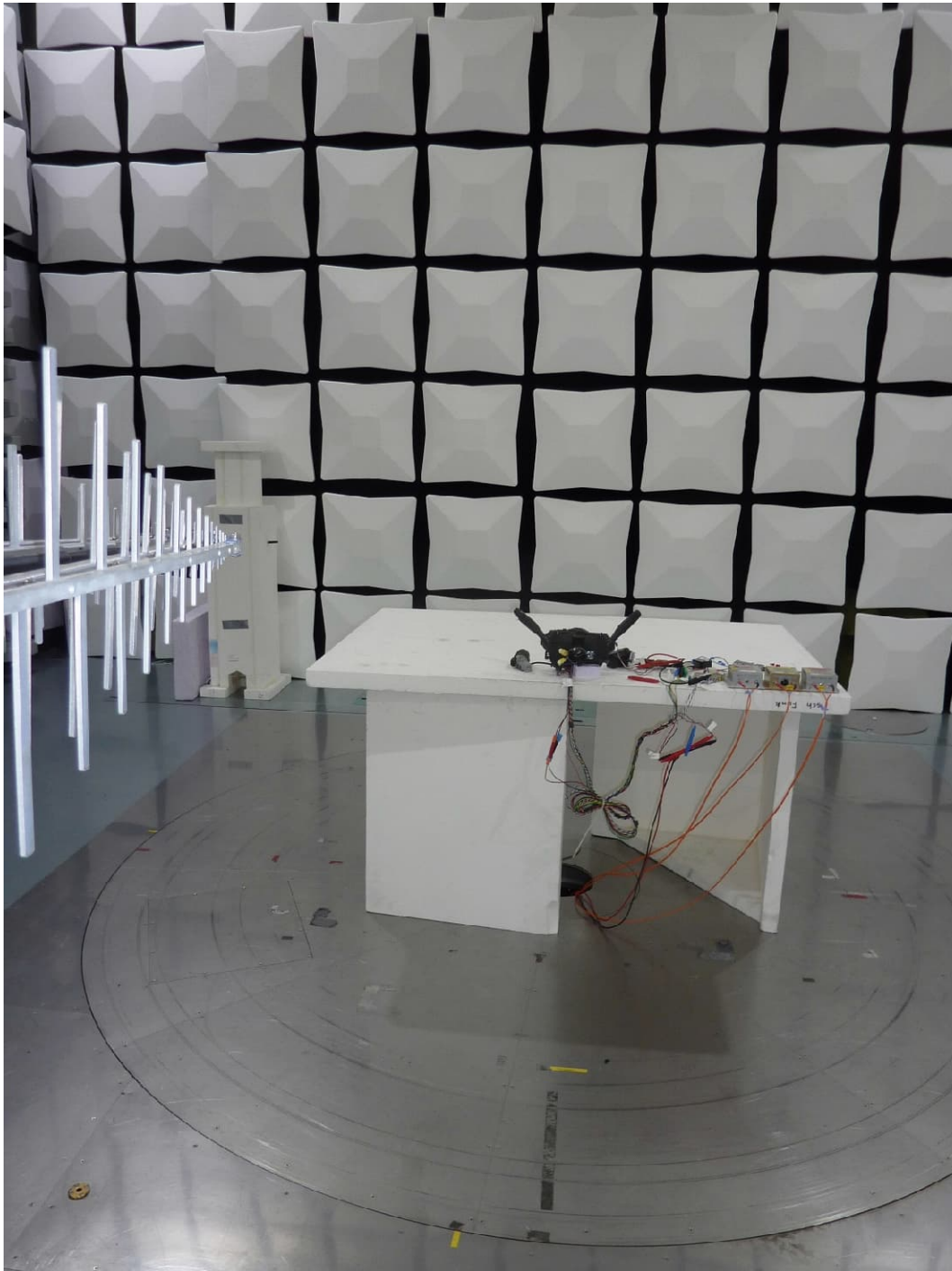
Test setup semi-anechoic chamber M276, 30 MHz – 1 GHz
