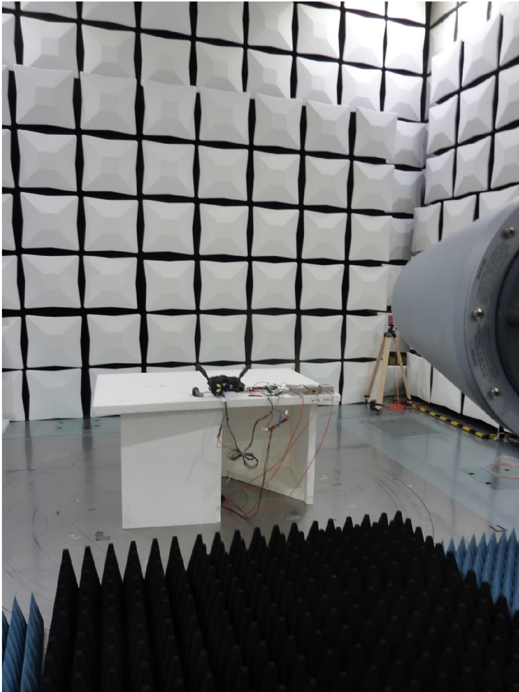
Test setup semi-anechoic chamber M276, 1 – 2 GHz
