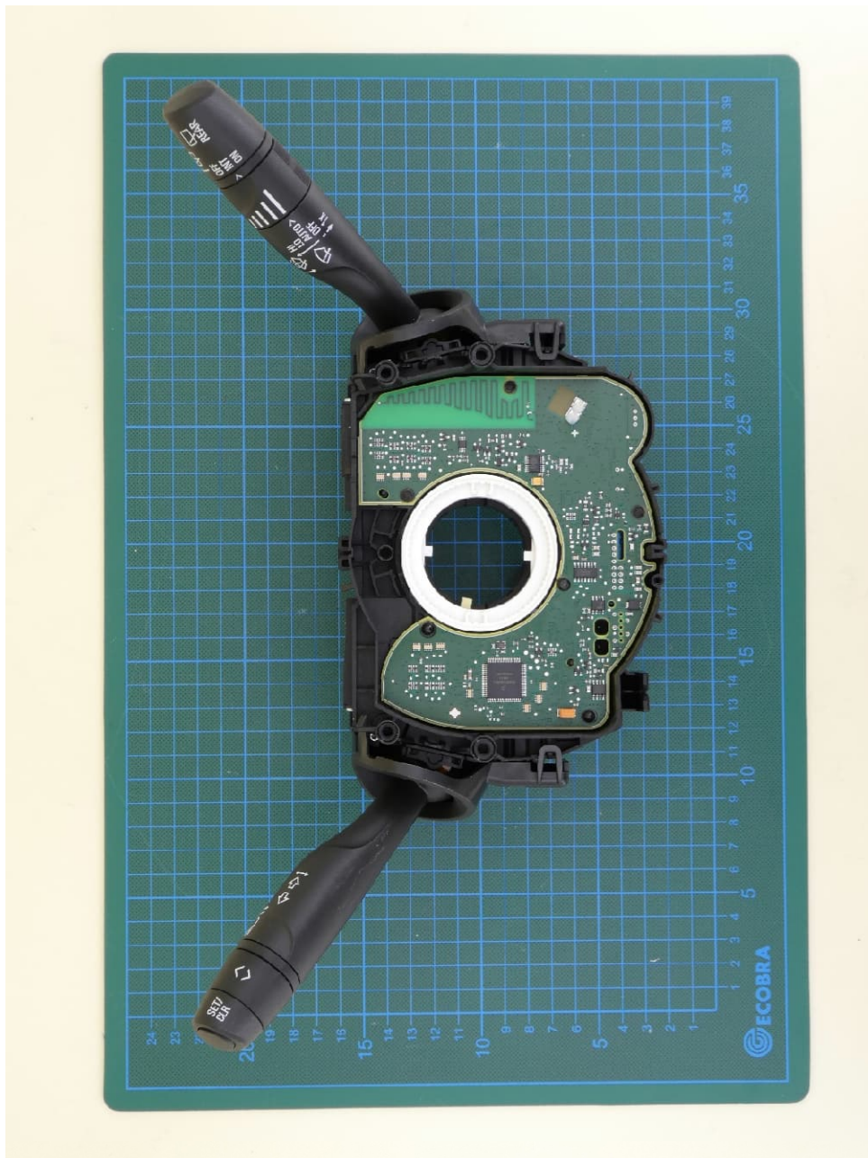
COM 2016 CEM2, internal view 2, housing opened
