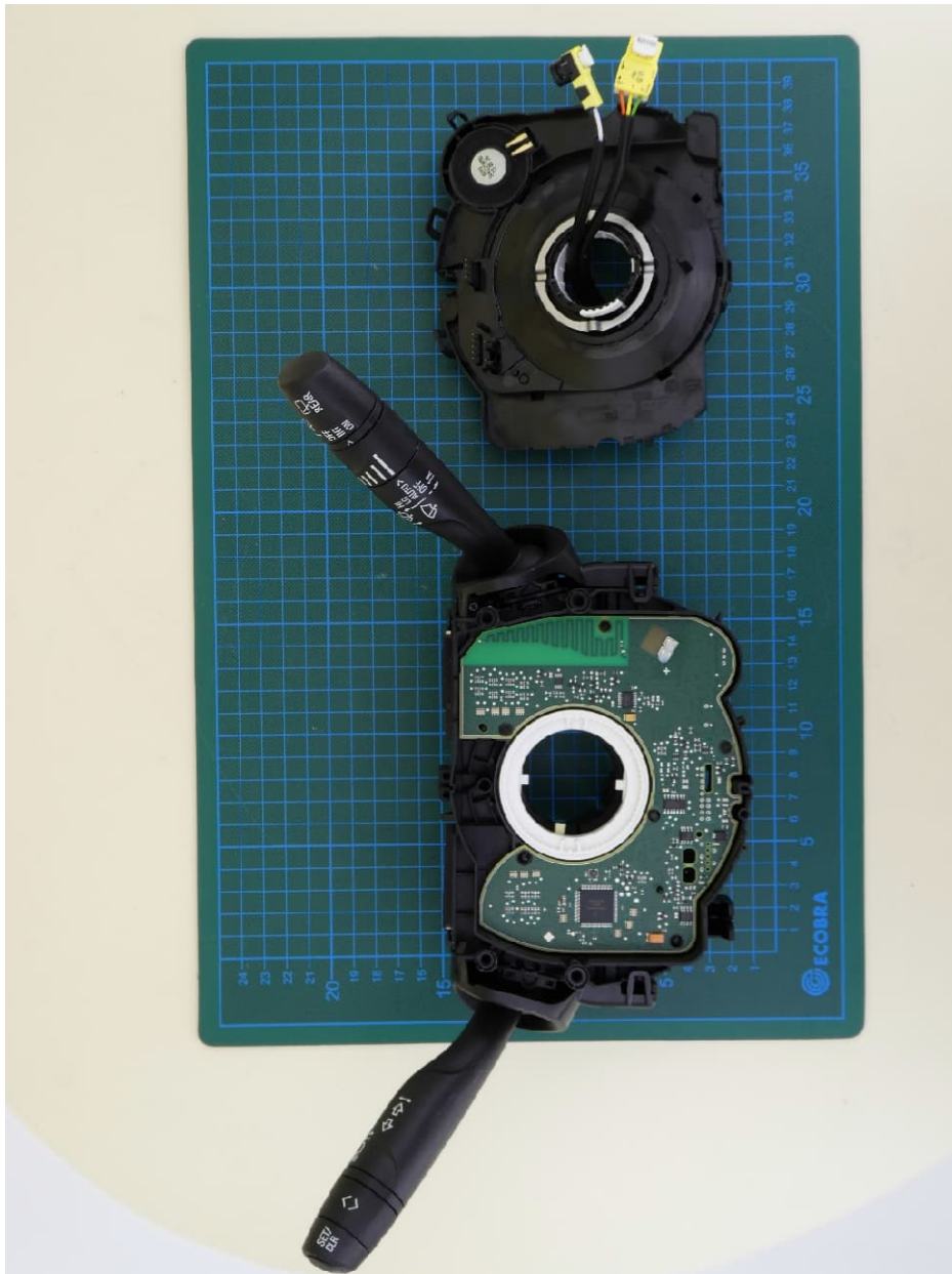
COM 2016 CEM2, internal view 1, housing opened
