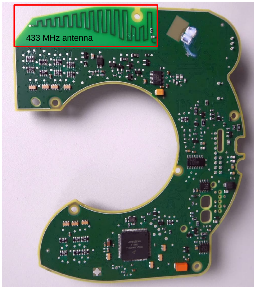
COM 2016 CEM2, PCB, top view
