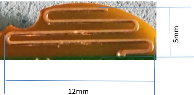
Picture of antenna
