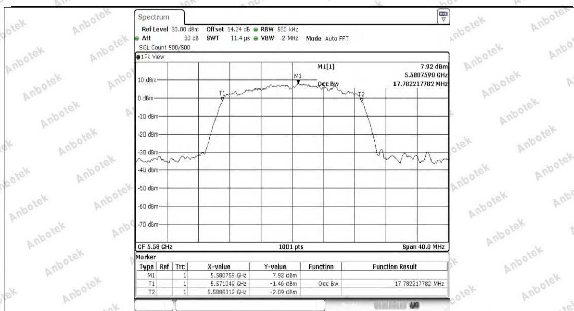
11AC20SISO-Ant1-5580
