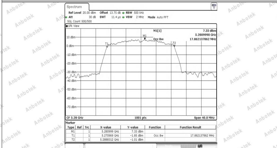
11AC20SISO-Ant1-5280
