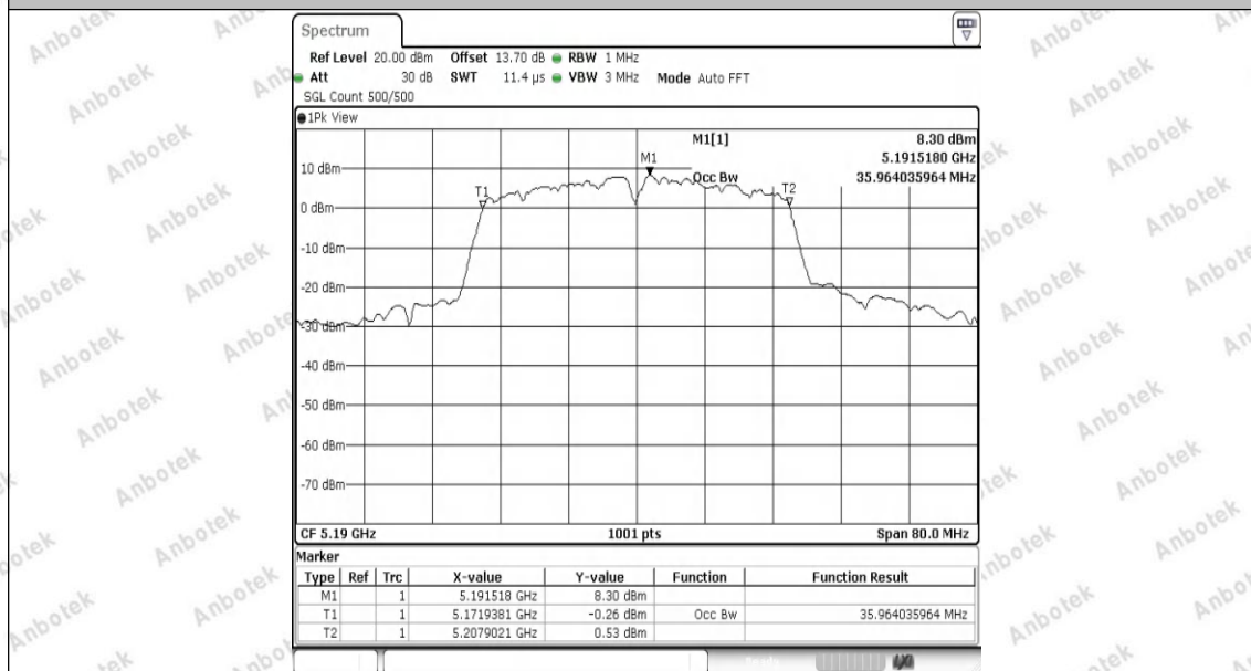
11AC40SISO-Ant1-5190
