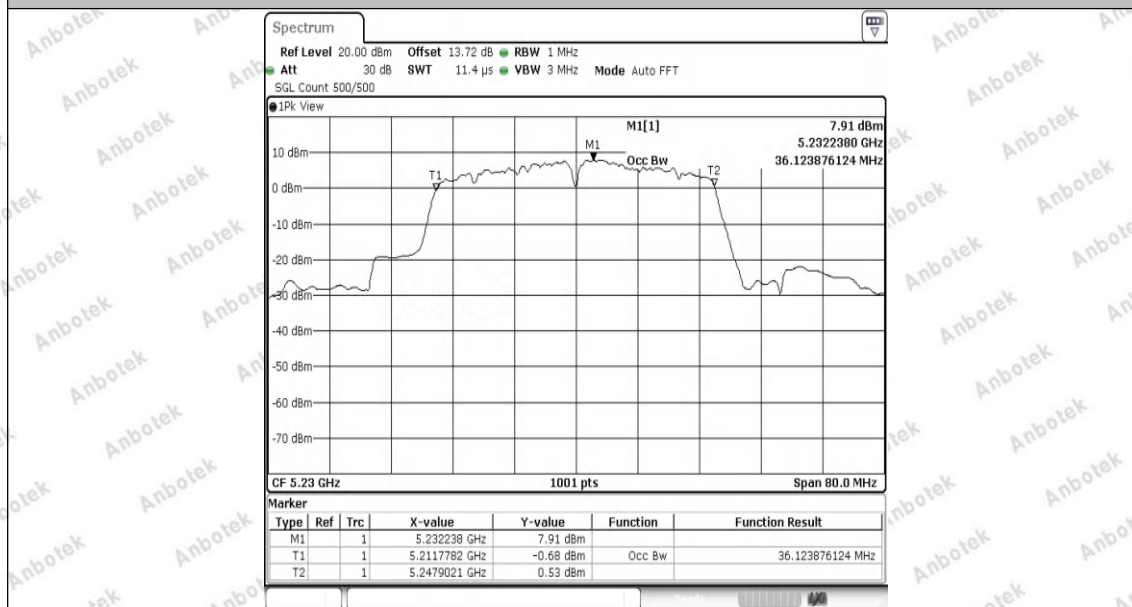
11N40SISO-Ant1-5230
