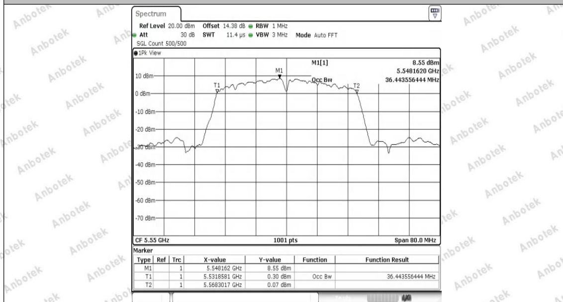
11N40SISO-Ant1-5550
