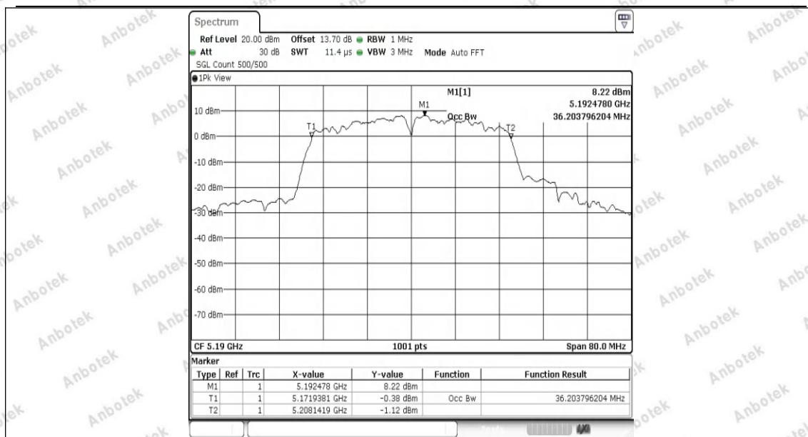
11N40SISO-Ant1-5190
