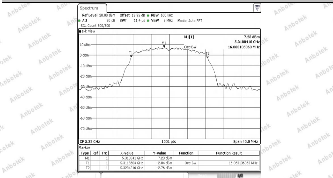
11A-Ant1-5320
