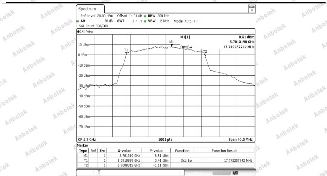
11N20SISO-Ant1-5700
