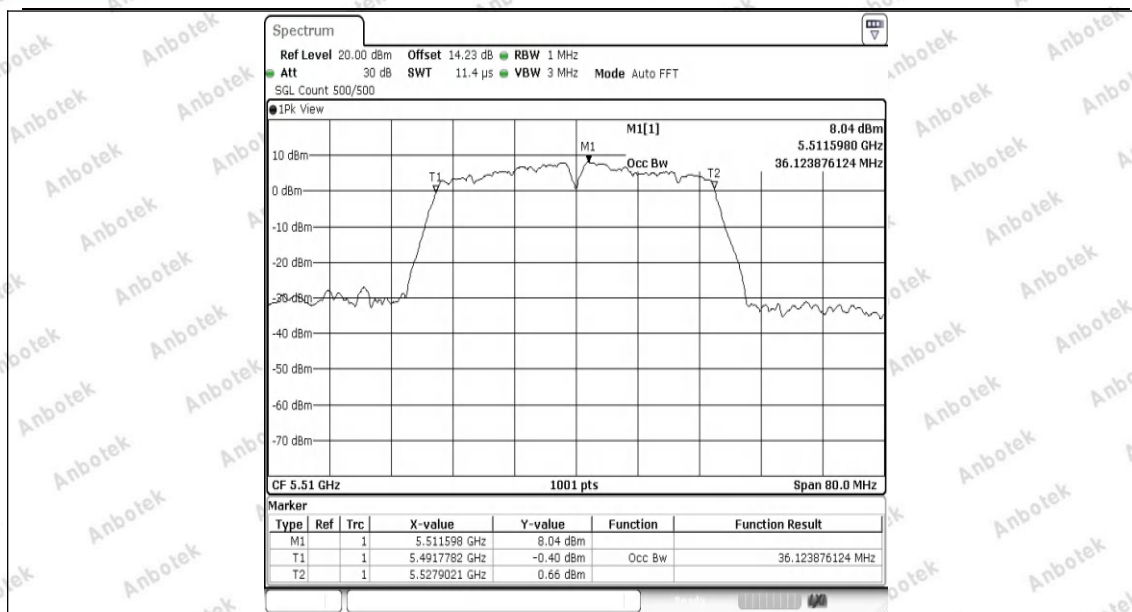
11N40SISO-Ant1-5510
