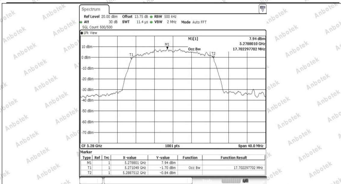
11N20SISO-Ant1-5280
