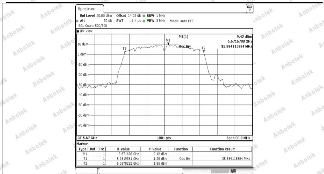
11N40SISO-Ant1-5670
