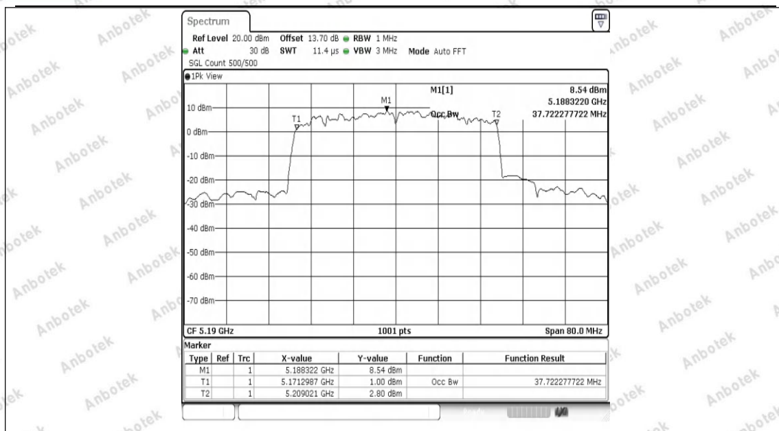
11AX40SISO-Ant1-5190
