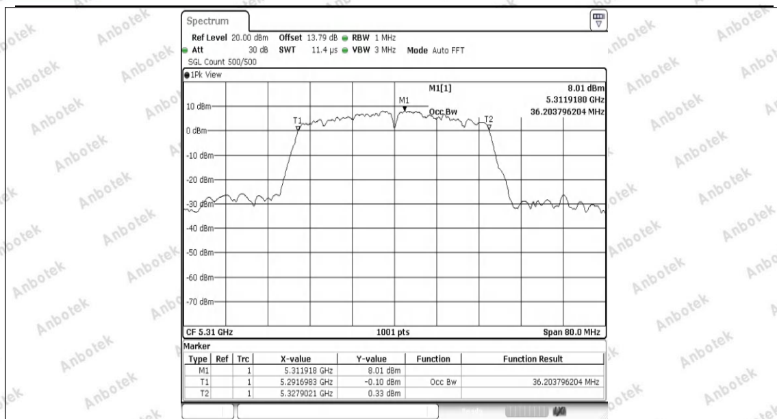
11AC40SISO-Ant1-5310
