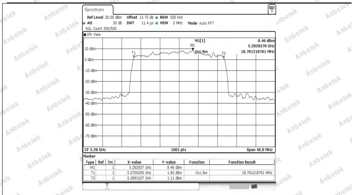
11AX20SISO-Ant1-5280
