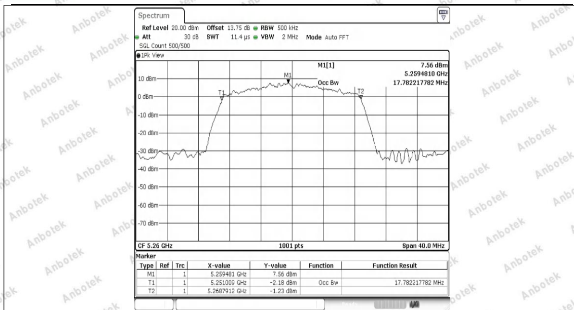
11AC20SISO-Ant1-5260
