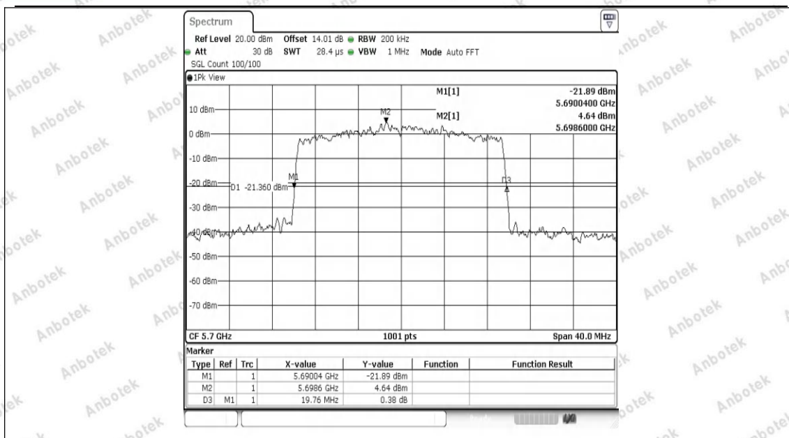
11AX20SISO-Ant1-5700
