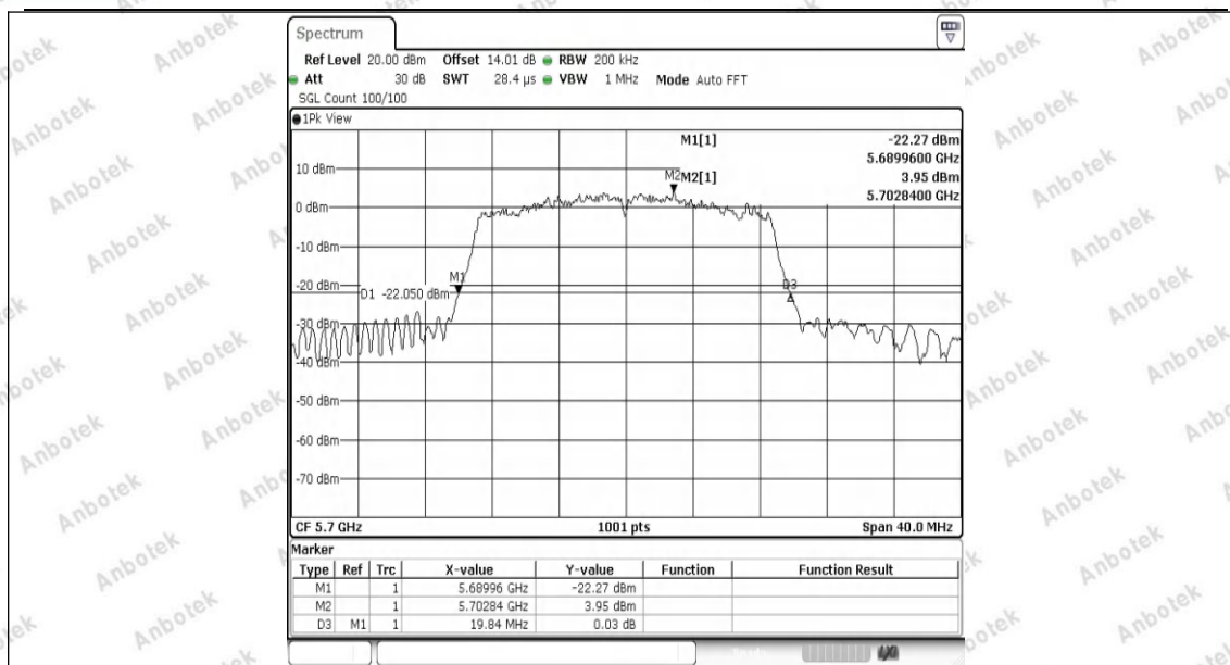
11N20SISO-Ant1-5700
