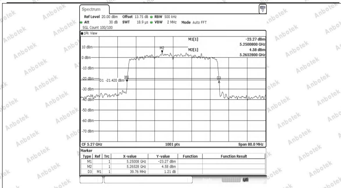
11AX40SISO-Ant1-5270
