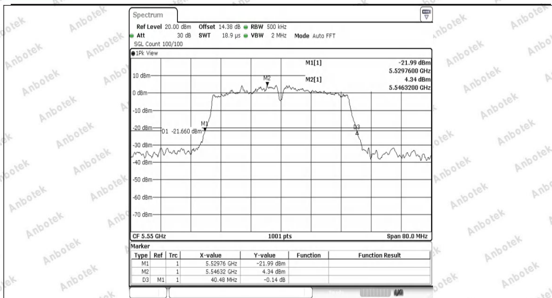
11AC40SISO-Ant1-5550
