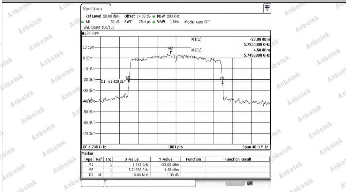
11AX20SISO-Ant1-5745
