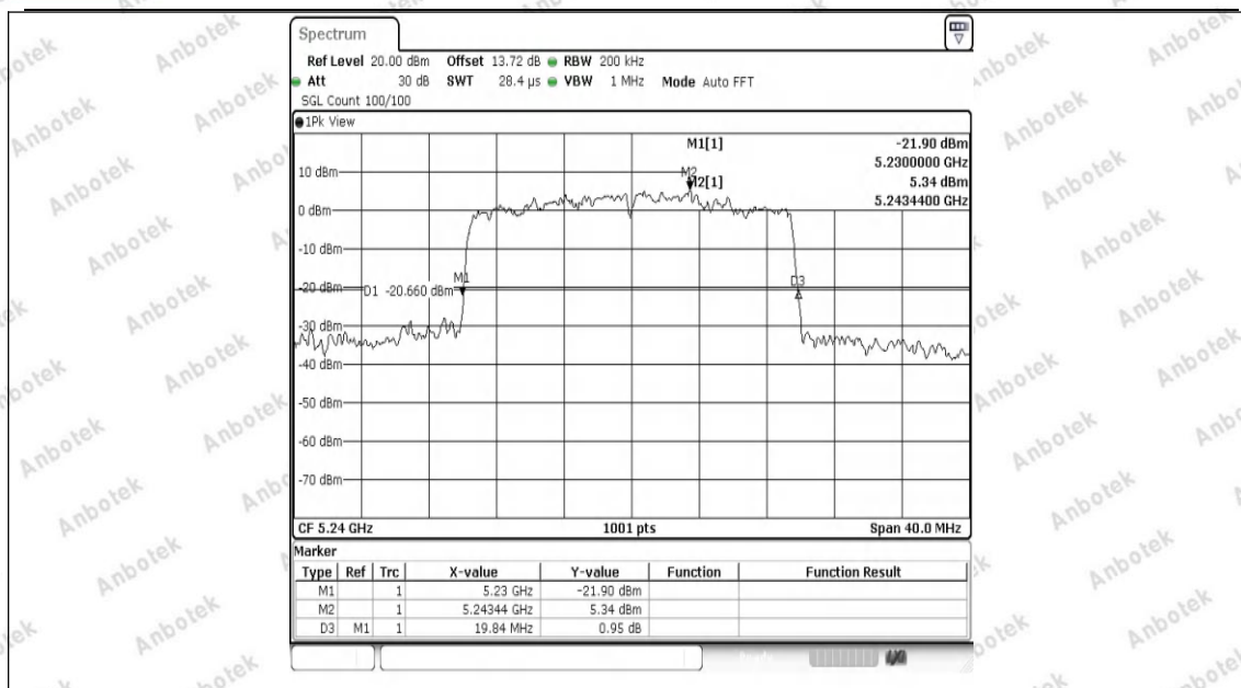
11AX20SISO-Ant1-5240
