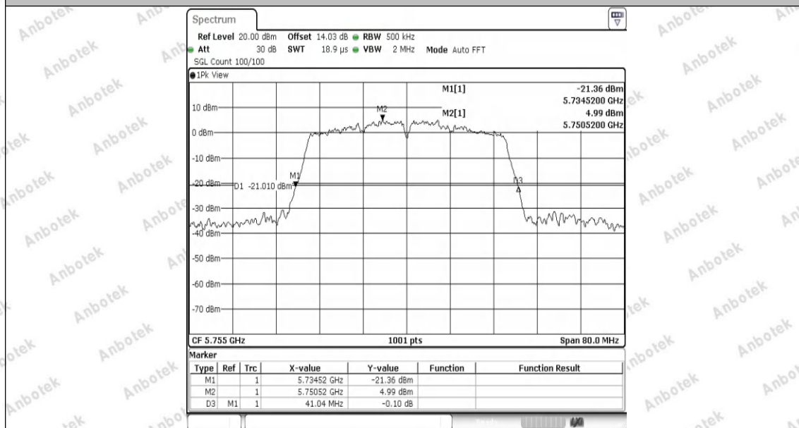
11N40SISO-Ant1-5755
