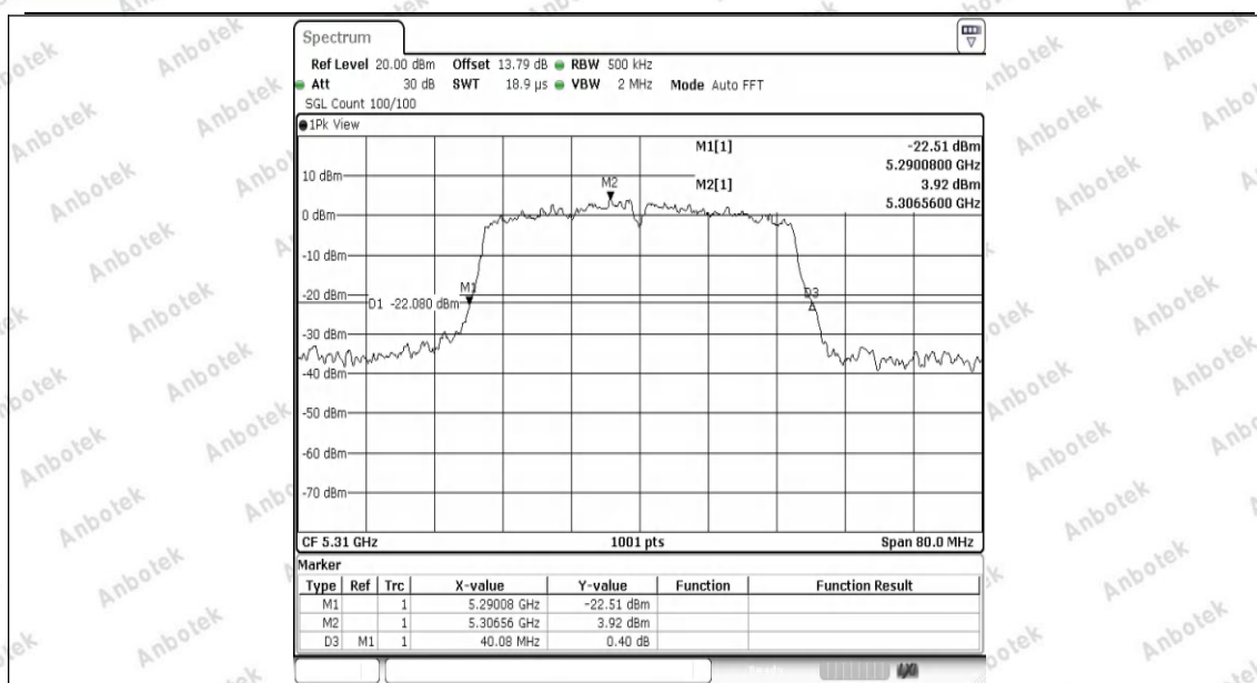
11AC40SISO-Ant1-5310
