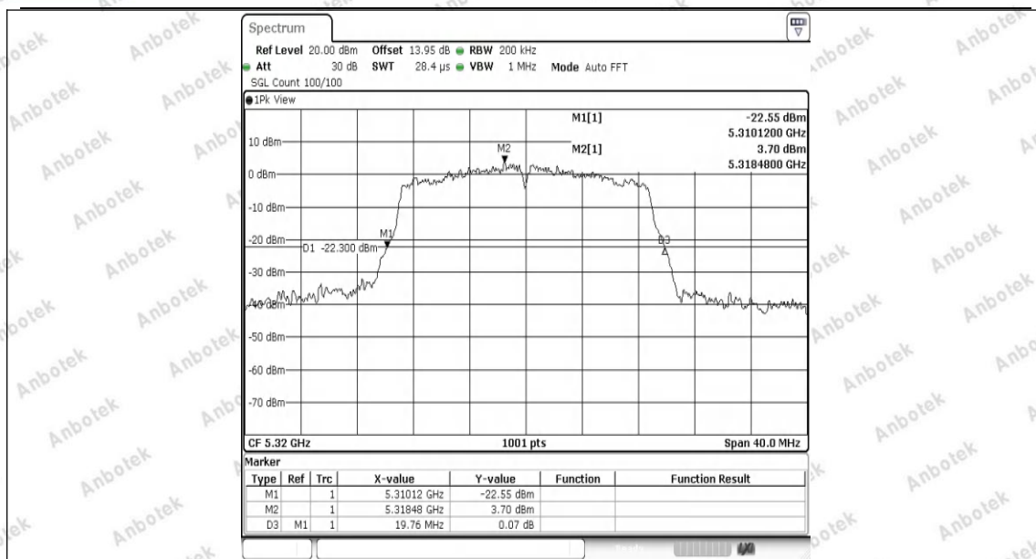
11AC20SISO-Ant1-5320
