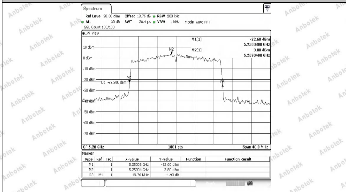
11AX20SISO-Ant1-5260
