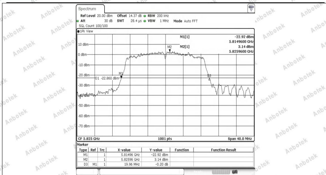
11AC20SISO-Ant1-5825
