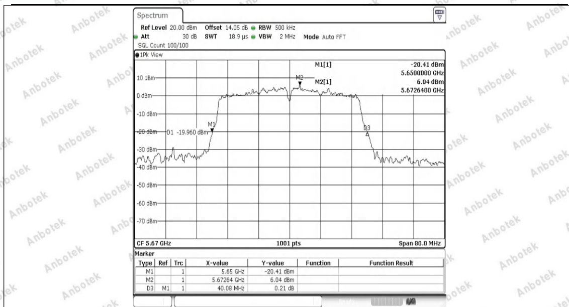
11N40SISO-Ant1-5670
