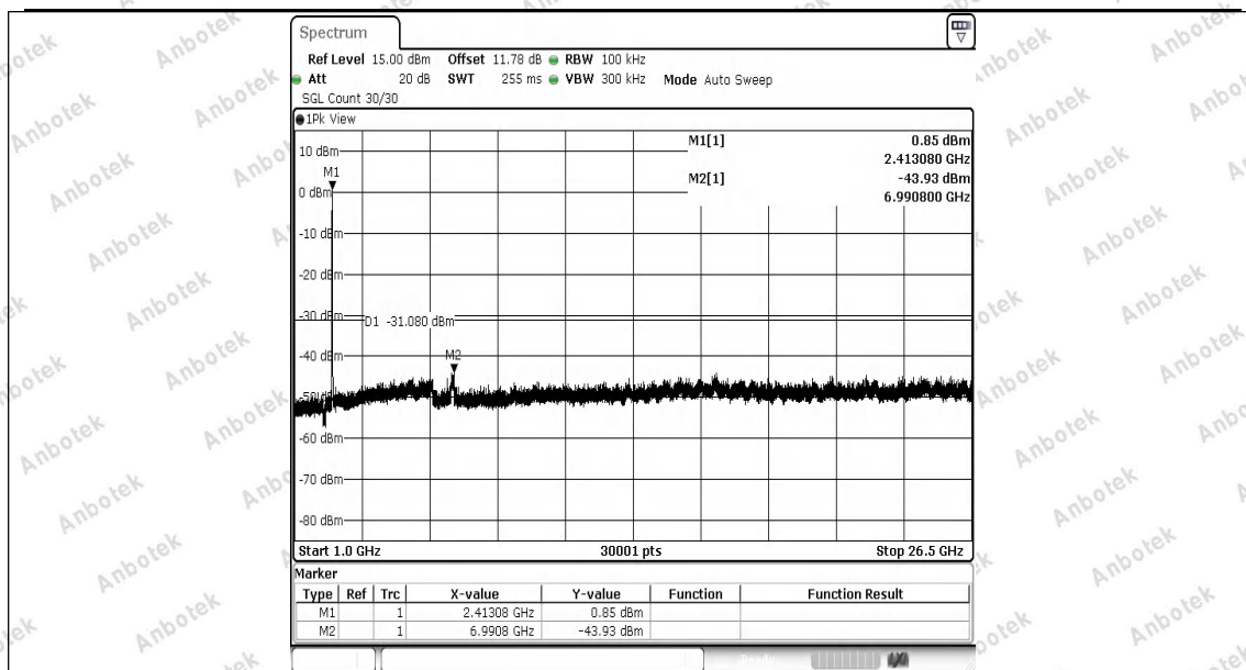
11AX20SISO-Ant1-2412-1000~26500-PASS
