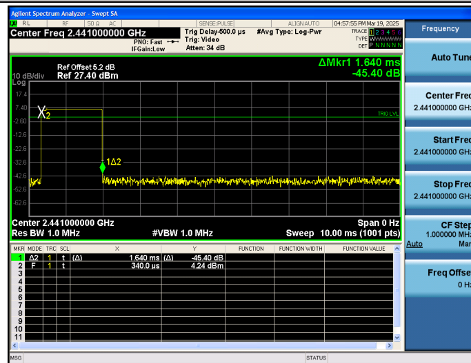
\pi/4 -DQPSK_2DH5_2441
