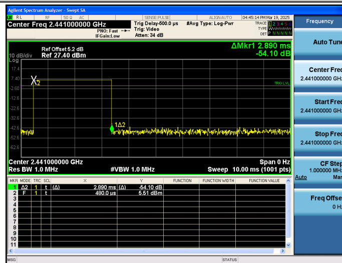
8-DPSK_3DH1_2441
