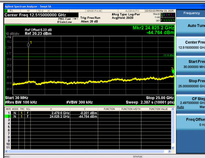
8-DPSK_2402_Reference
