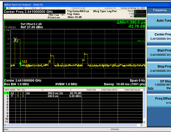
\pi/4 -DQPSK_2DH3_2441
