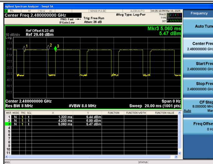
8-DPSK_2480
