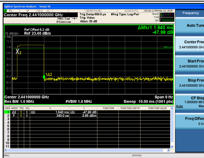
8-DPSK_3DH5_2441
