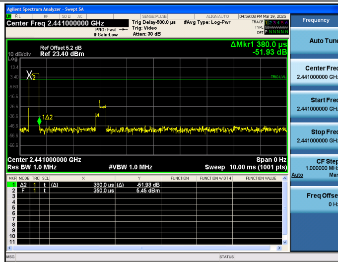
8-DPSK_3DH3_2441
