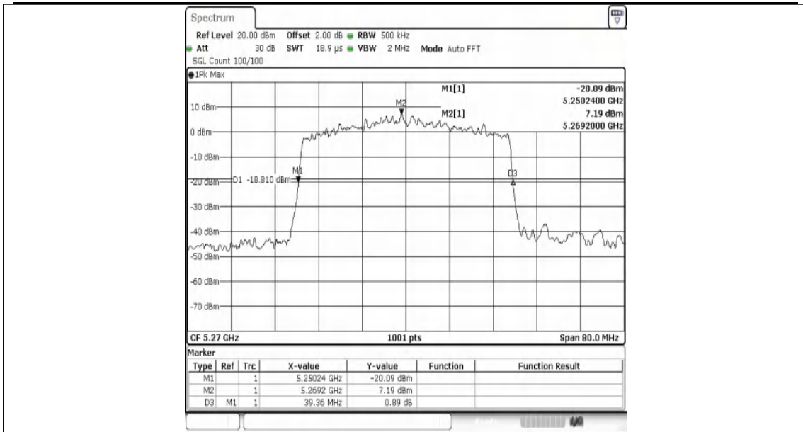
11AX40SISO-Ant1-5270
