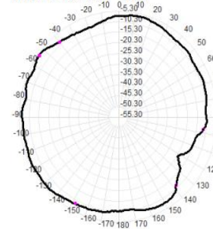
2410.0MHz Total(E2), Max=-5.99dBi
