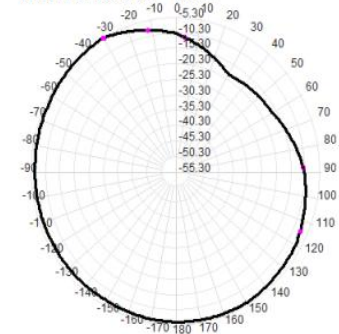
2410.0MHz Total(H), Max=-5.30dBi
