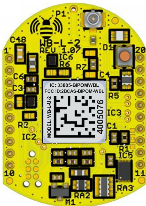
Top marking for WB-L-U-2
