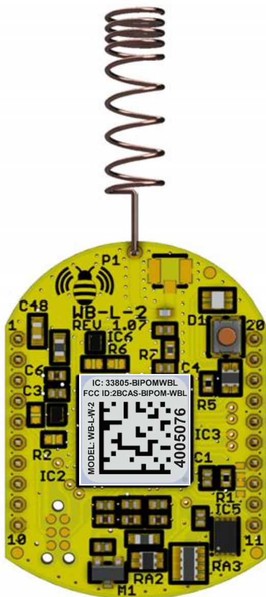
Top marking for WB-L-W-2
