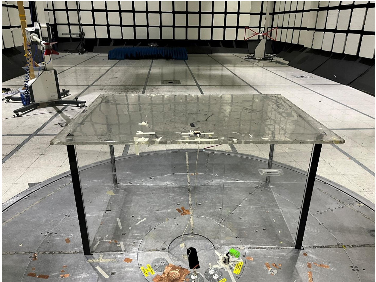
Radiated Emissions, 30MHz – 1GHz, Rear View
