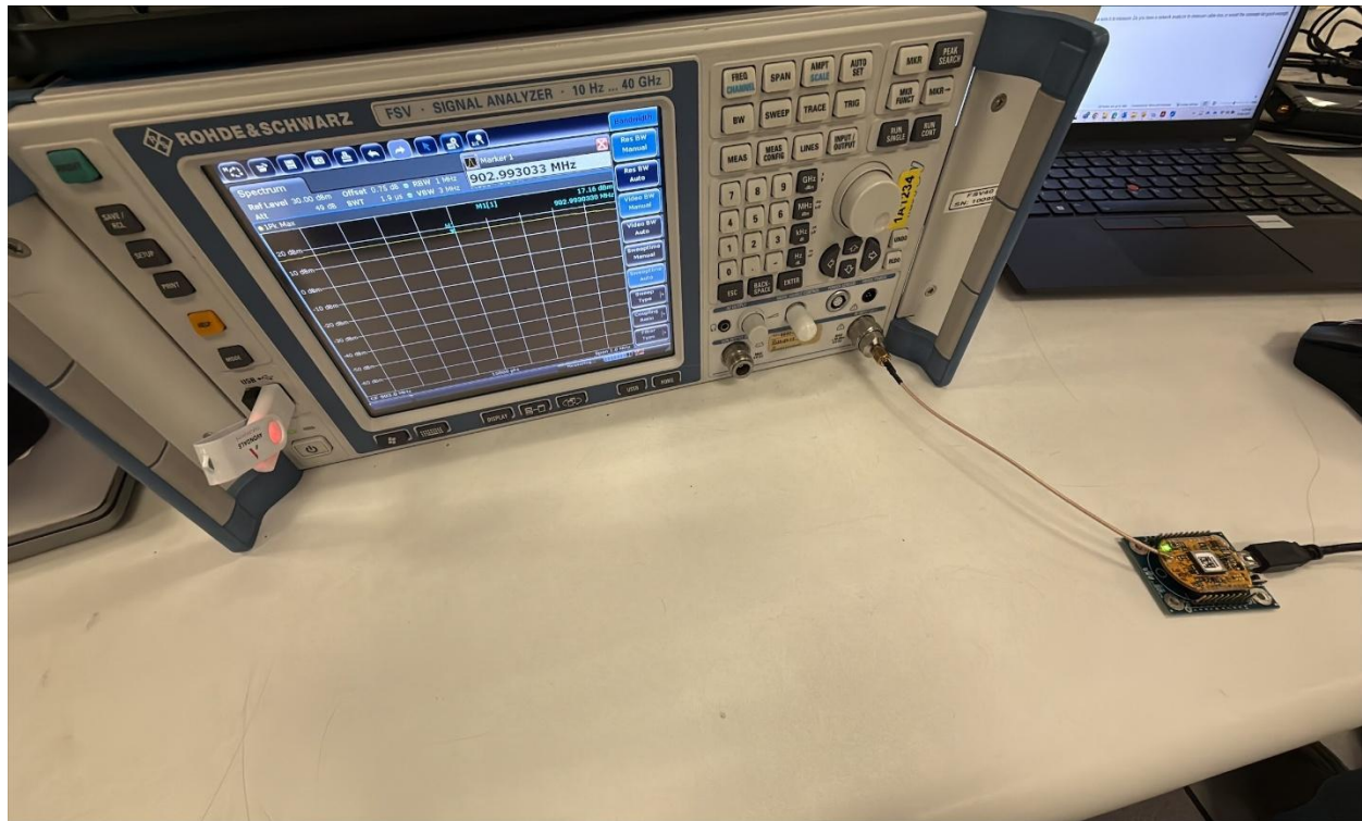
Conducted Antenna Port Testing
