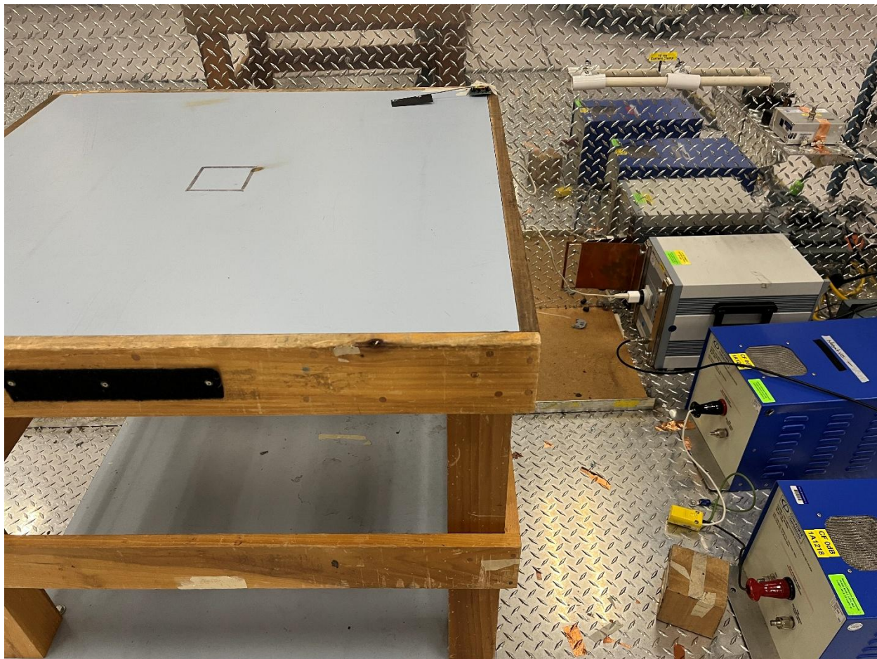
Conducted Emissions at AC Mains (Front Side)
