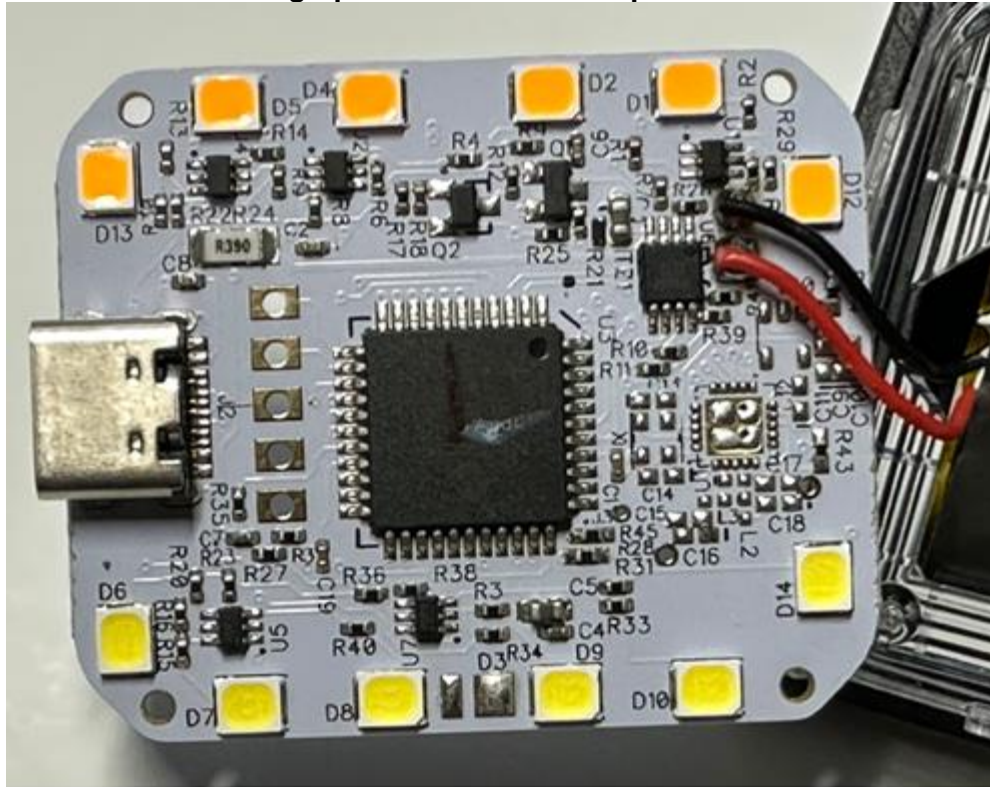
Photograph of PC Board: Component Side
