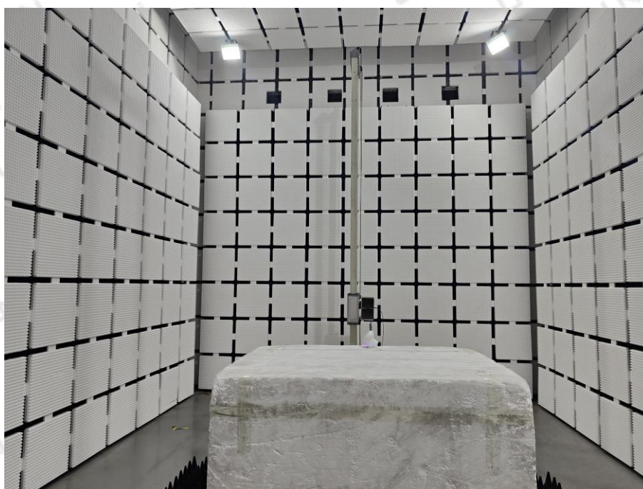
Above 1GHz
