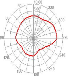
Bluetooth 0 TRP H
