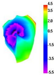
Bluetooth 39 TRP
