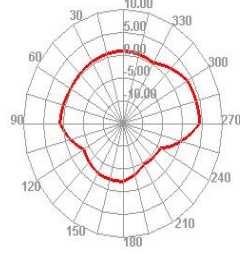
Bluetooth 19 TRP H
