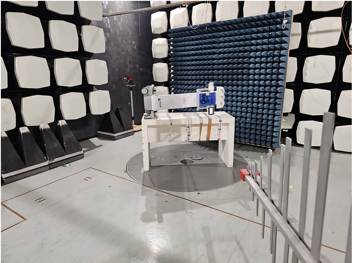
Fig. Mea.: 5 : SAC measurement > 30 MHz
