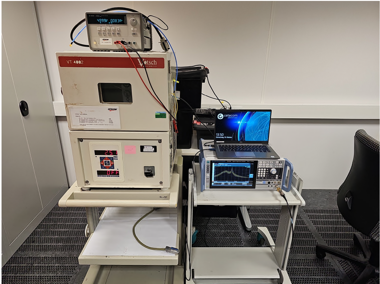
Fig. Mea.: 6 : Climatic test; overview
