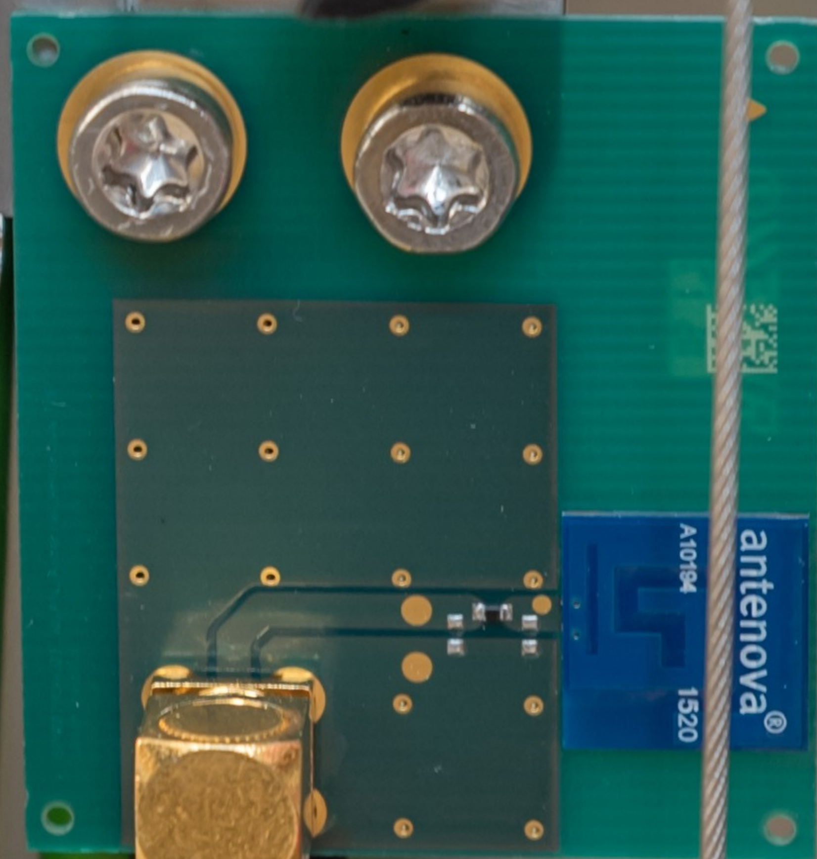
Antenna of ublox ELLA-W131
