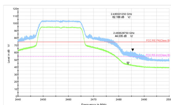
802.11g-Channel 10 Peak+ Average
