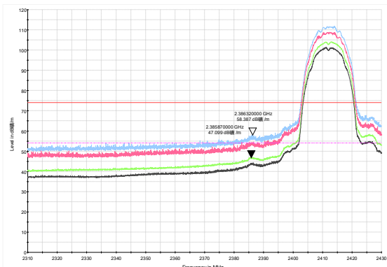
802.11b-Channel 1 Peak+ Average
