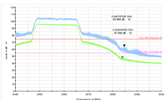
802.11n HT20-Channel 10 Peak+ Average
