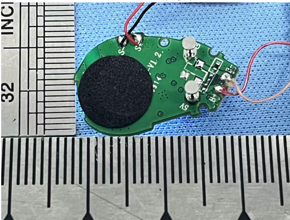
Internal Photos(Right)
