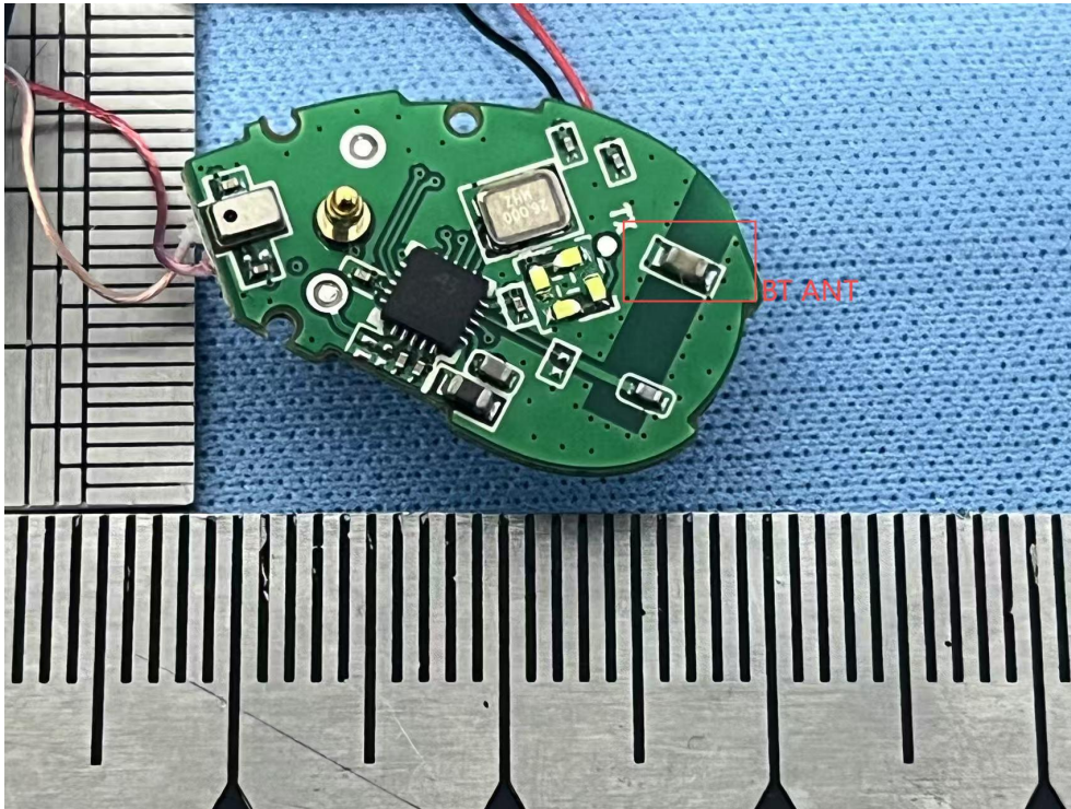
Internal Photos(Right)
