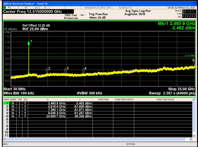
Spurious Emission IEEE 802.11g Channel 11 20MHz Antenna 0
