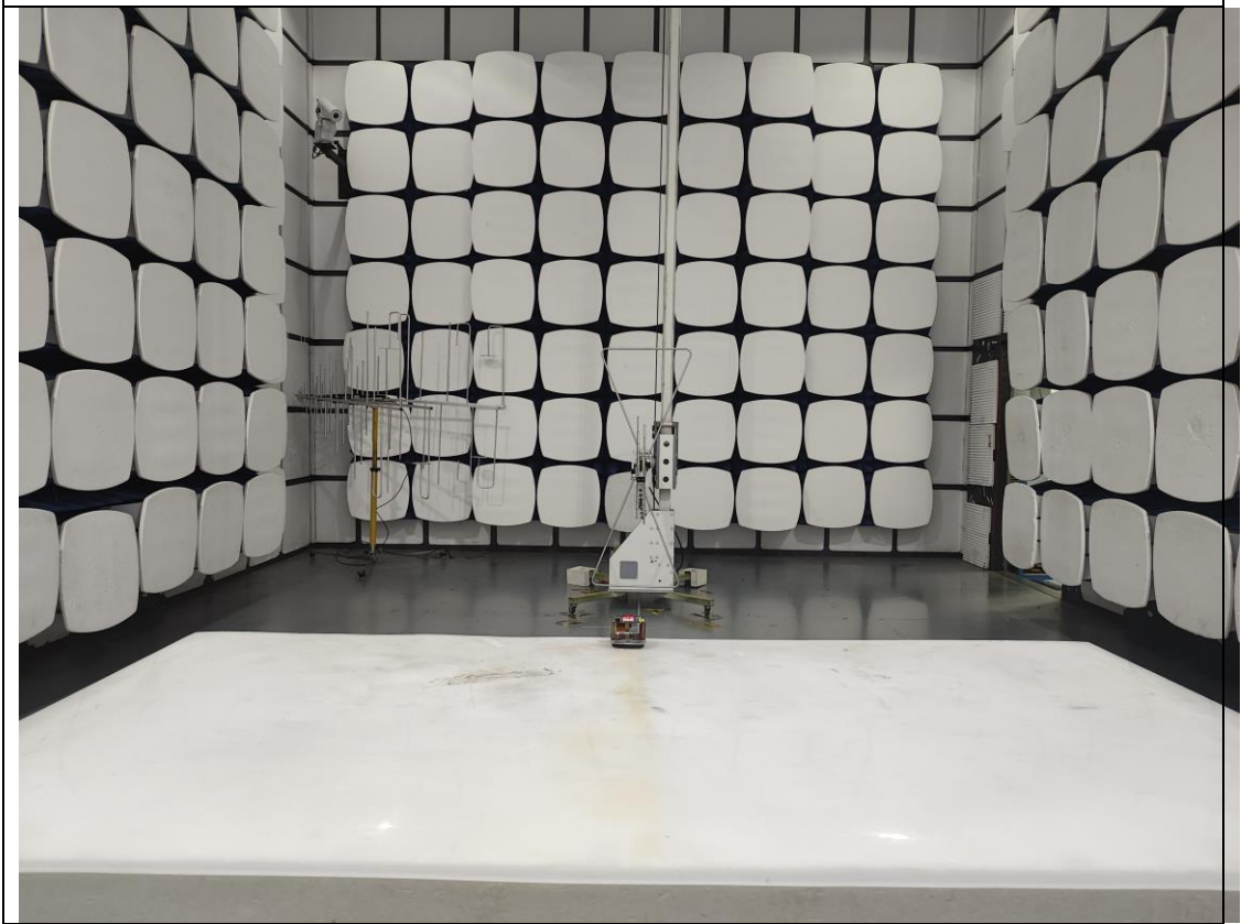
Radiated Emission
