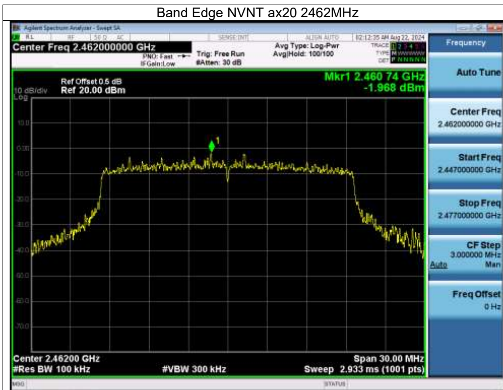
Band Edge NVNT ax20 2462MHz Emission
