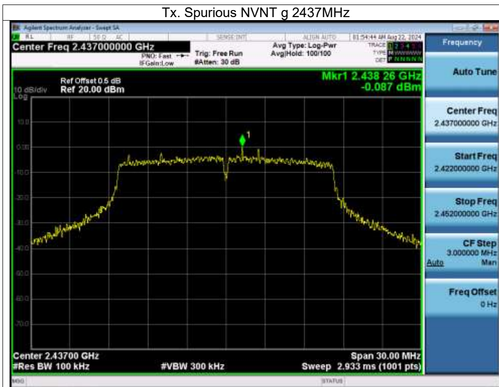
Tx. Spurious NVNT g 2437MHz Emission
