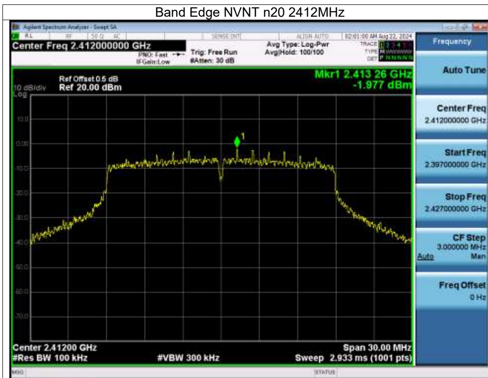
Band Edge NVNT n20 2412MHz Emission
