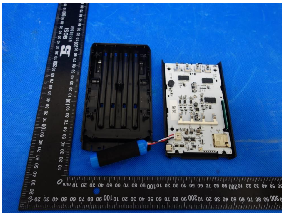
Figure 4: Internal view (Device Base of model WT06)
