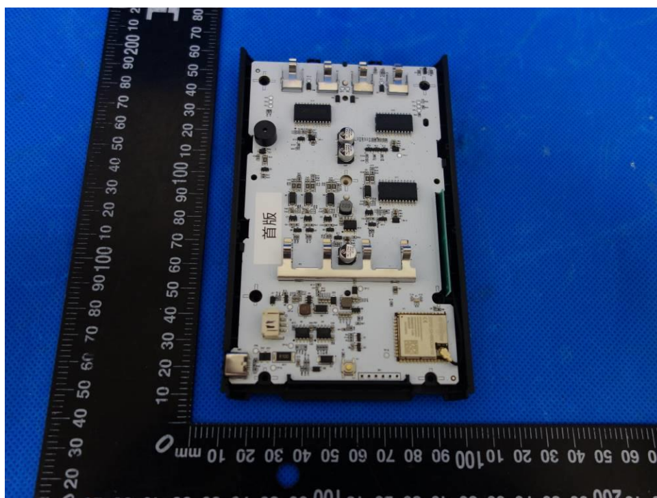
Figure 6: Internal view (Device Base of model WT06)
