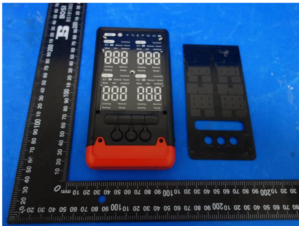
Figure 1: Internal view (Device Base and Probe of model WT06)
