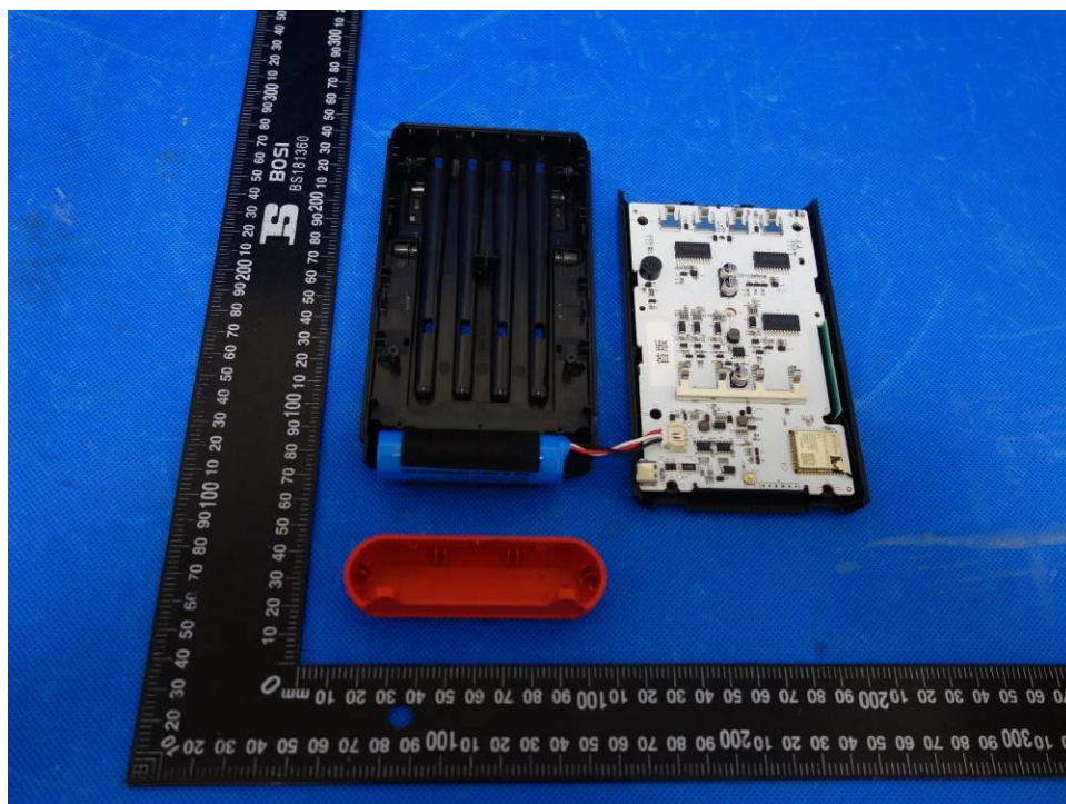
Figure 3: Internal view (Device Base of model WT06)
