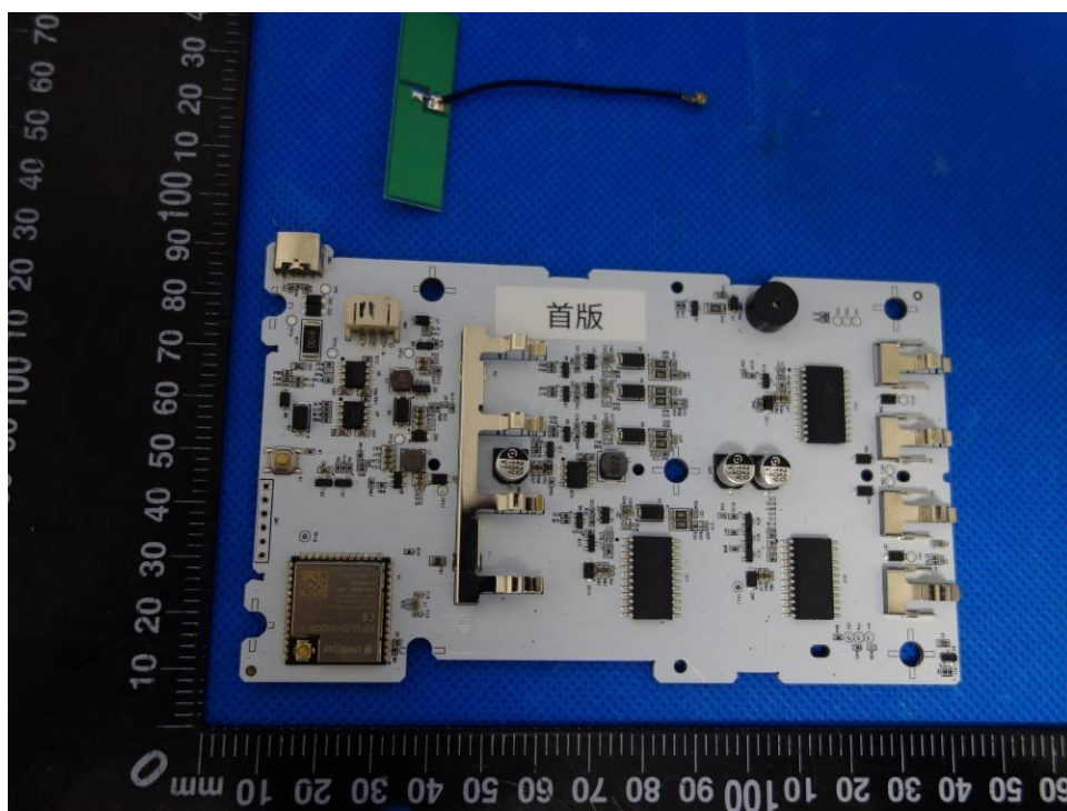
Figure 8: Main PCB (Device Base of model WT06)
