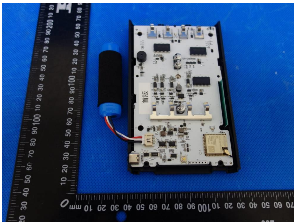
Figure 5: Internal view (Device Base of model WT06)
