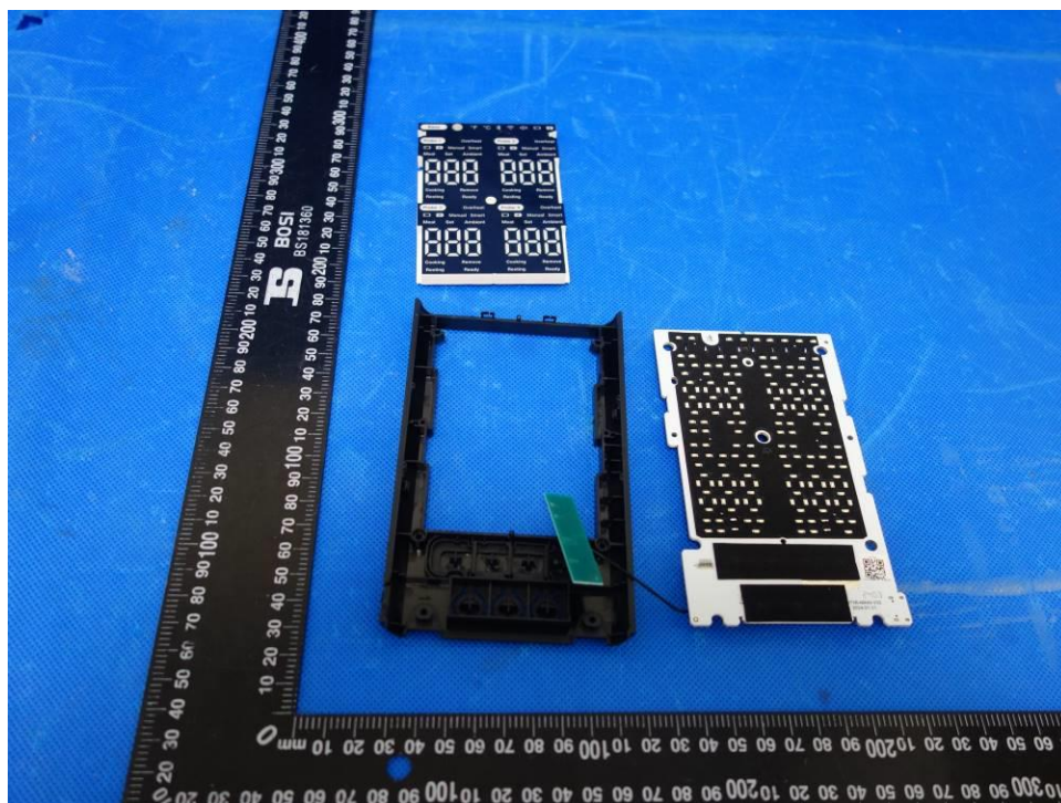
Figure 7: Internal view (Device Base of model WT06)
