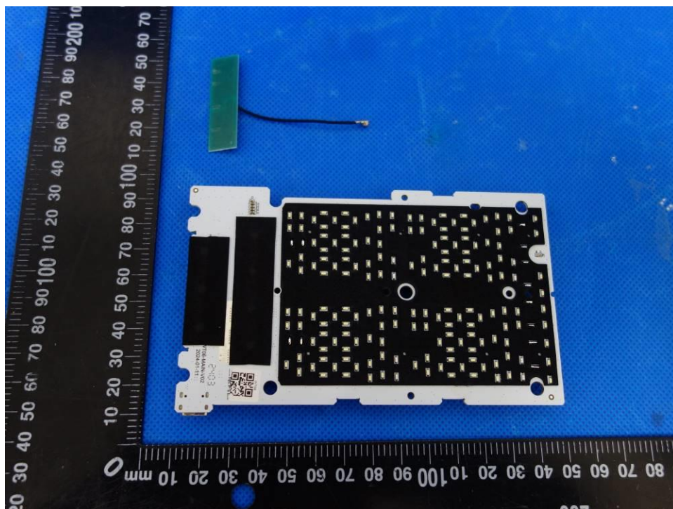
Figure 9: Main PCB (Device Base of model WT06)
