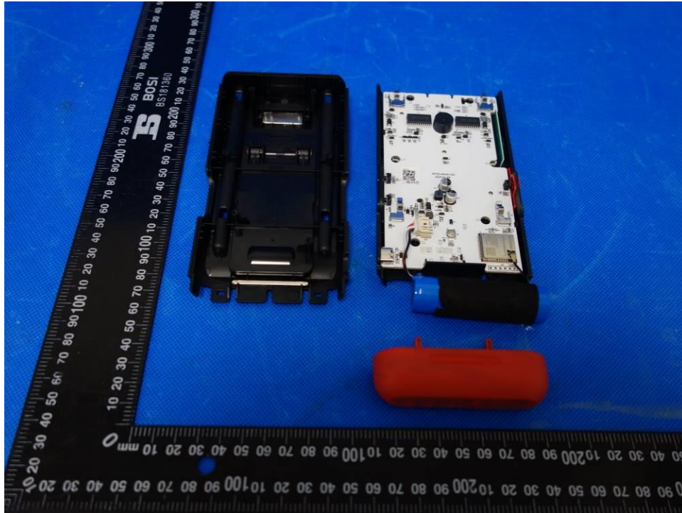
Figure 3: Internal view (Device Base of model WT02)
