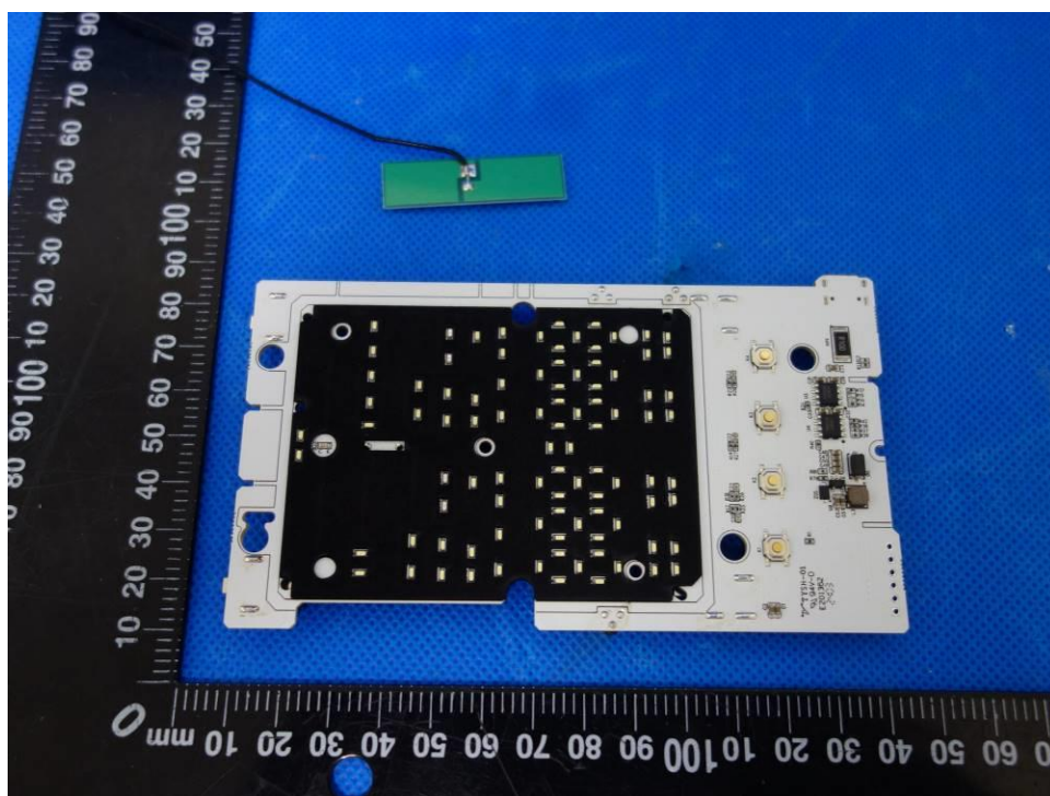
Figure 8: PCB view (Device Base of model WT02)
