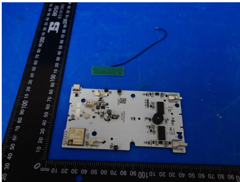
Figure 7: PCB view (Device Base of model WT02)
