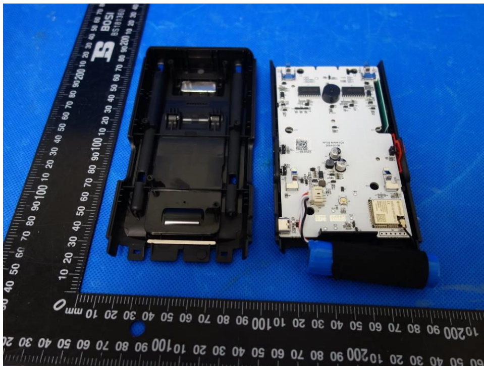
Figure 4: Internal view (Device Base of model WT02)
