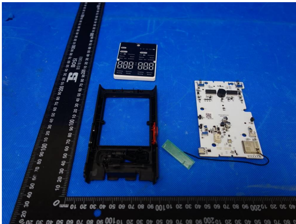
Figure 6: Internal view (Device Base of model WT02)
