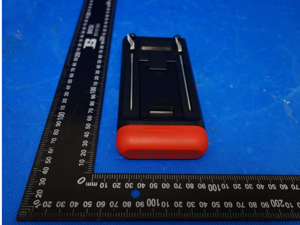
Figure 3: Overview (Device Base and Probe of model WT02)
