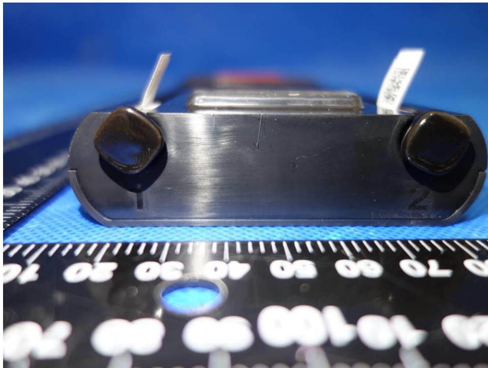
Figure 8: Overview (Device Base and Probe of model WT02)
