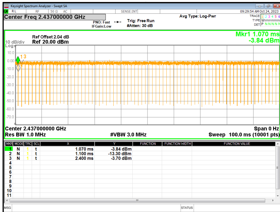
Duty Cycle NTV n20 2437MHz Ant1
