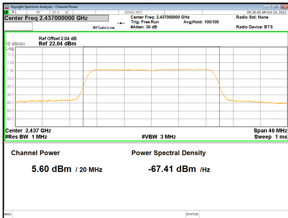
Average Power NTV n20 2437MHz Ant1
