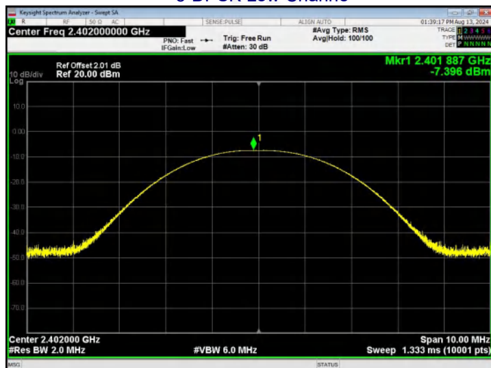
8-DPSK Low Channe
