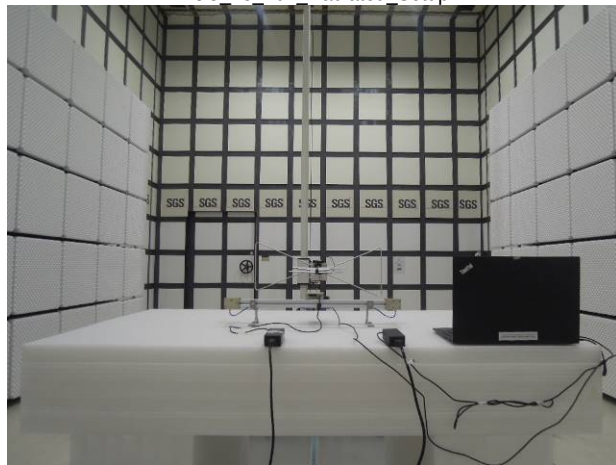
FCC 15 407 Radiated Setup
