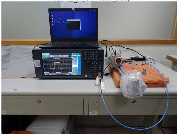
FCC 15 407 Normal CBP Setup
