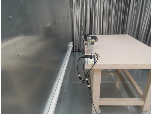
FCC 15 407 Conduction Setup
