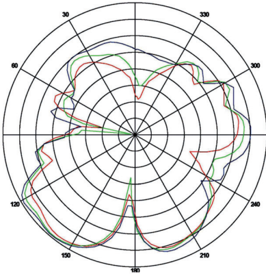
Horizontal: 2400 MHz 2450 MHz 2500 MHz Power (dBm) Max: 0 Min: -40 Scale: 5/div
