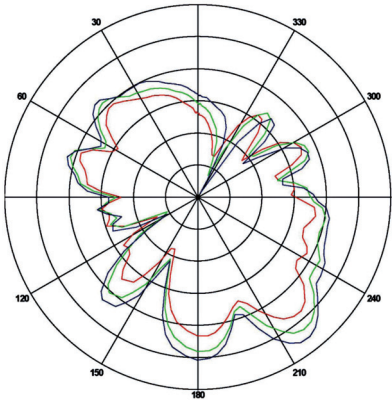
Vertical: 2400 MHz 2450 MHz 2500 MHz Power (dBm) Max: 0 Min: -30 Scale: 5/div
