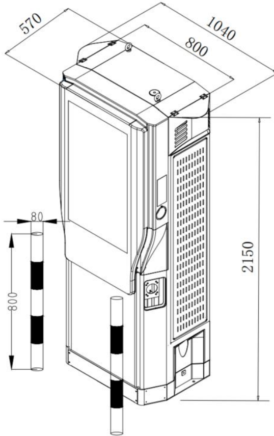
Fig. 5-1 Dimensions of SONEIL SPARK
