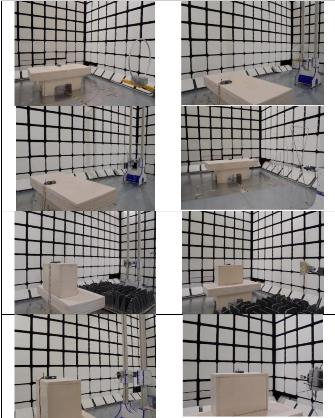
Radiated Emissions Test setup
