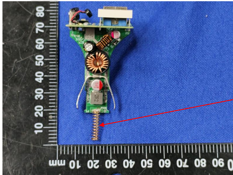
FM Antenna
