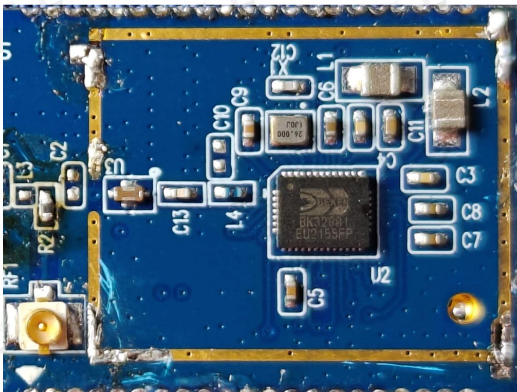
Bluetooth antenna model: C4207-810023-A(SSR-2400194)-x3
