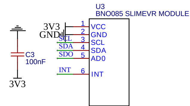
Main Board Connection
