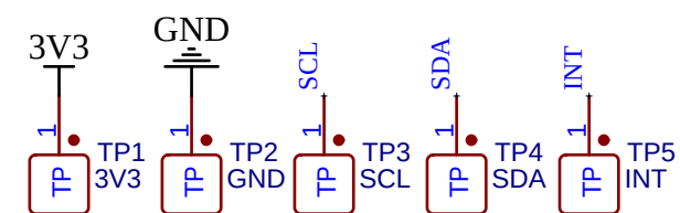
Test Points
