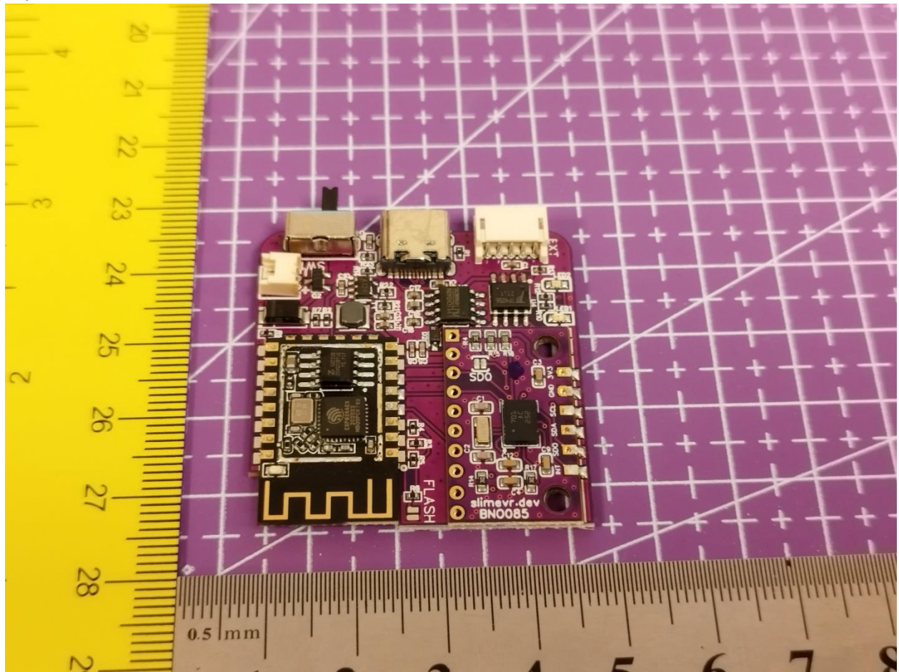
Top view, wireless module without the lid:
