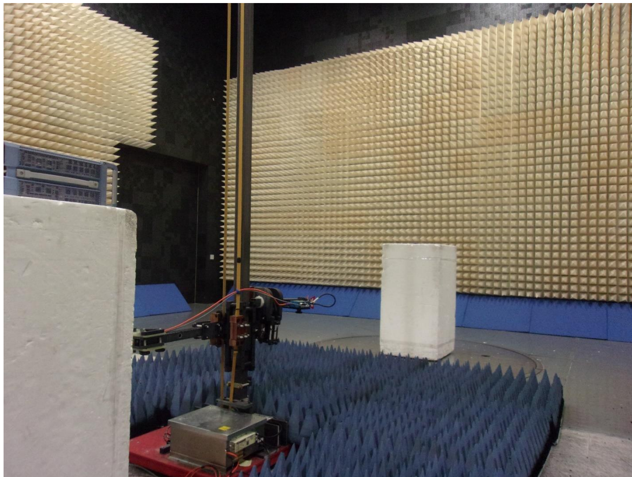
Radiated Spurious Emissions, 18 GHz – 40 GHz
