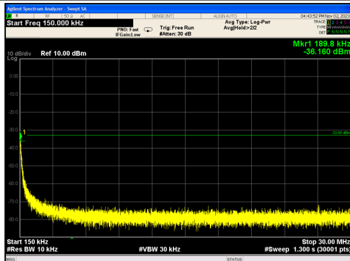
Band66_1.4MHz_QPSK_131979_1RB#5
