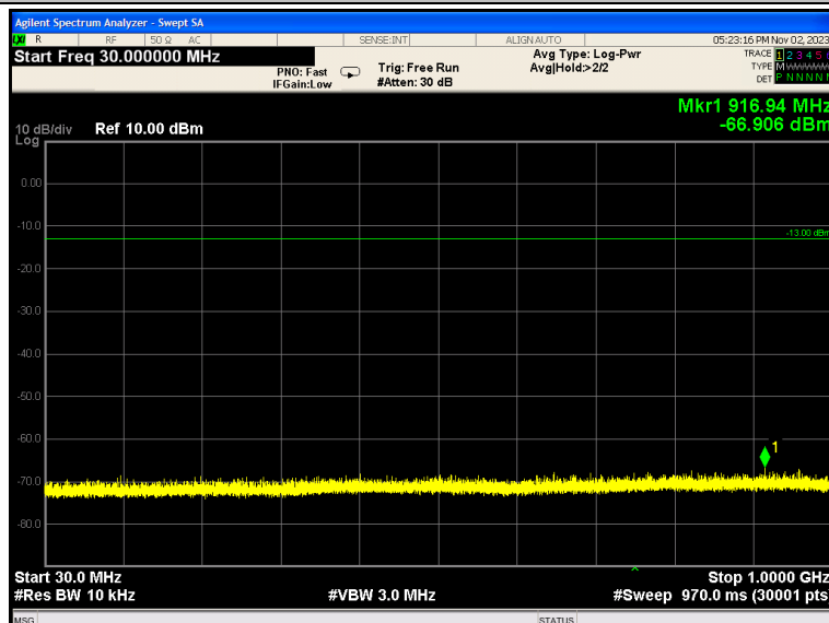
Band66_1.4MHz_QPSK_131979_1RB#5
