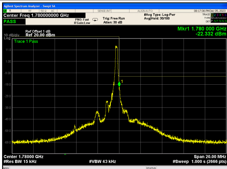
Band66-1.4MHz-QPSK-132665-1RB#5
