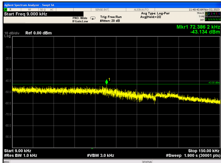
Band66_1.4MHz_QPSK_131979_1RB#5
