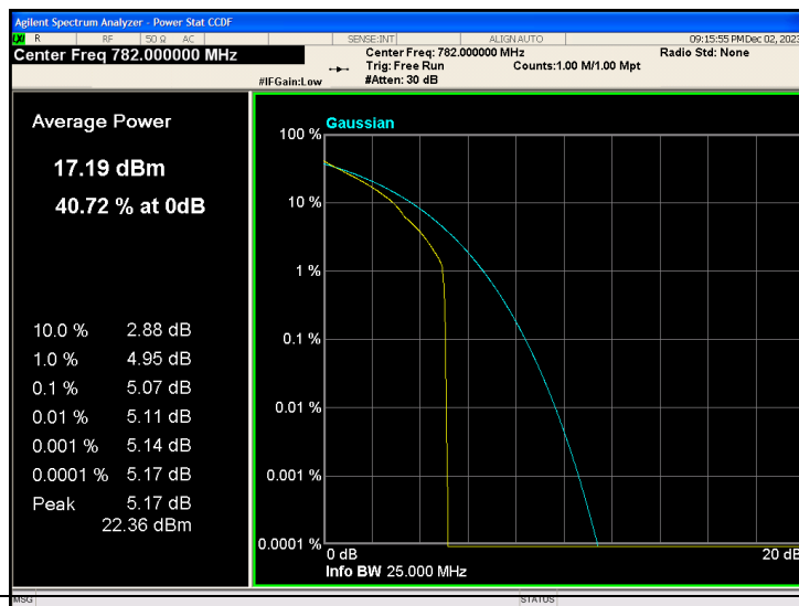
Band13_5MHz_QPSK_23230_1RB#0
