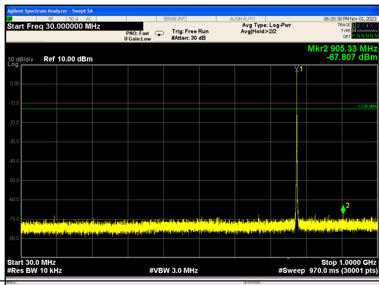
Band13_5MHz_QPSK_23205_1RB#12
