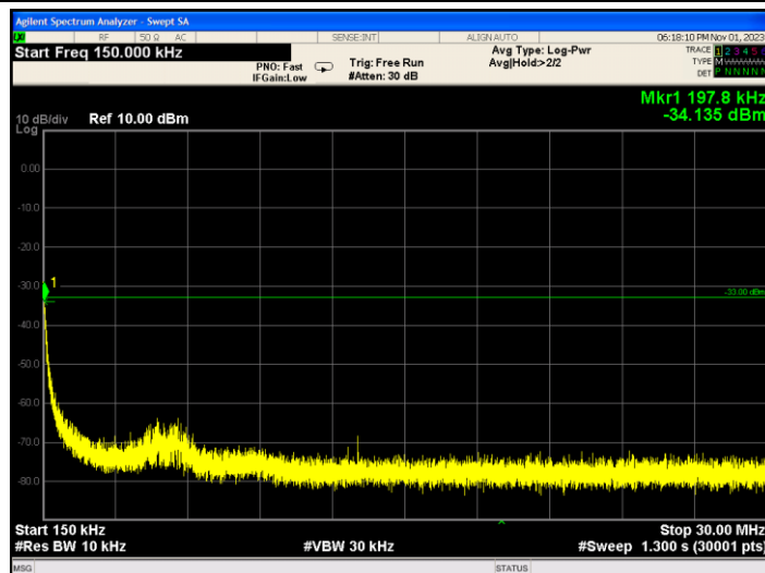
Band13_5MHz_QPSK_23205_1RB#12
