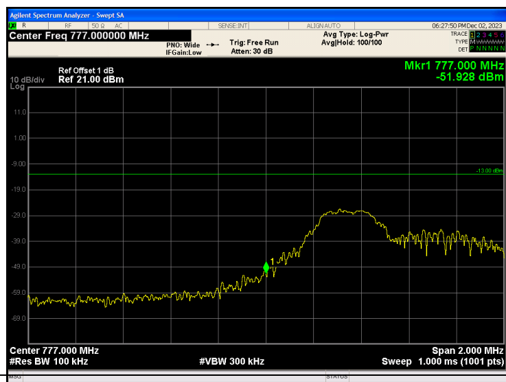
Band13_5MHz_QPSK_23205_1RB#24
