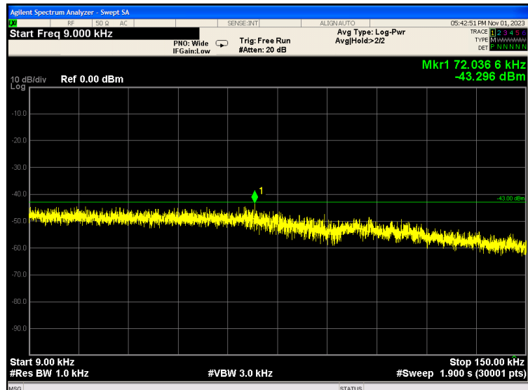
Band13_5MHz_QPSK_23205_1RB#12
