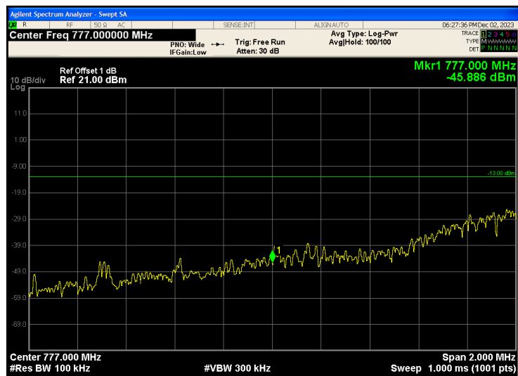
Band13_5MHz_QPSK_23205_1RB#24
