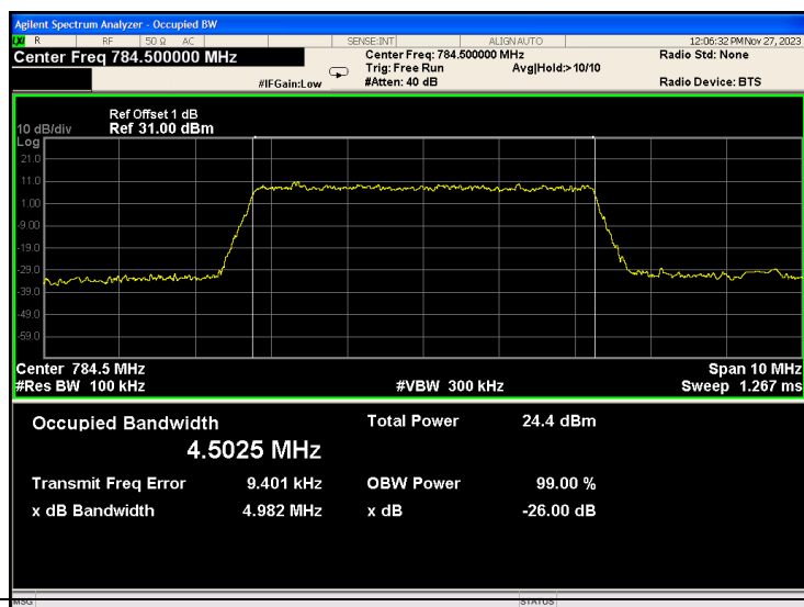
Band13_5MHz_QPSK_23255_25RB#0
