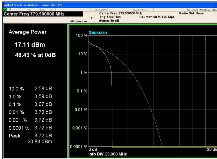
Band13_5MHz_QPSK_23205_25RB#0
