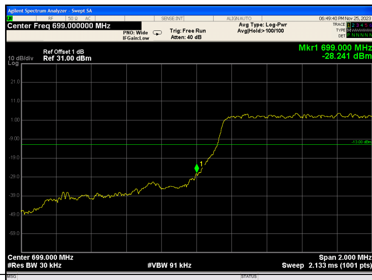
Band12-1.4MHz-QPSK-23017-6RB#0
