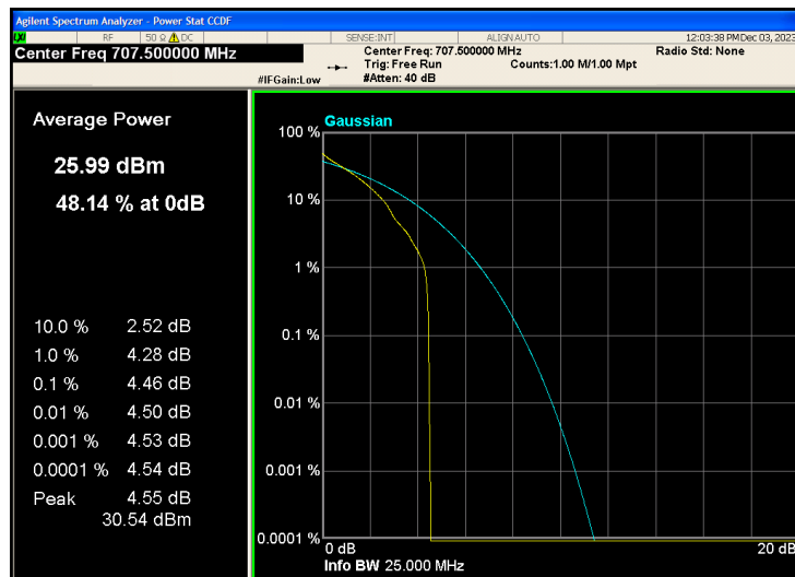
Band12-1.4MHz-QPSK-23095-1RB#0
