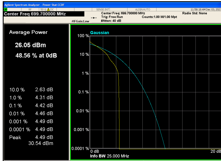
Band12-1.4MHz-QPSK-23017-6RB#0
