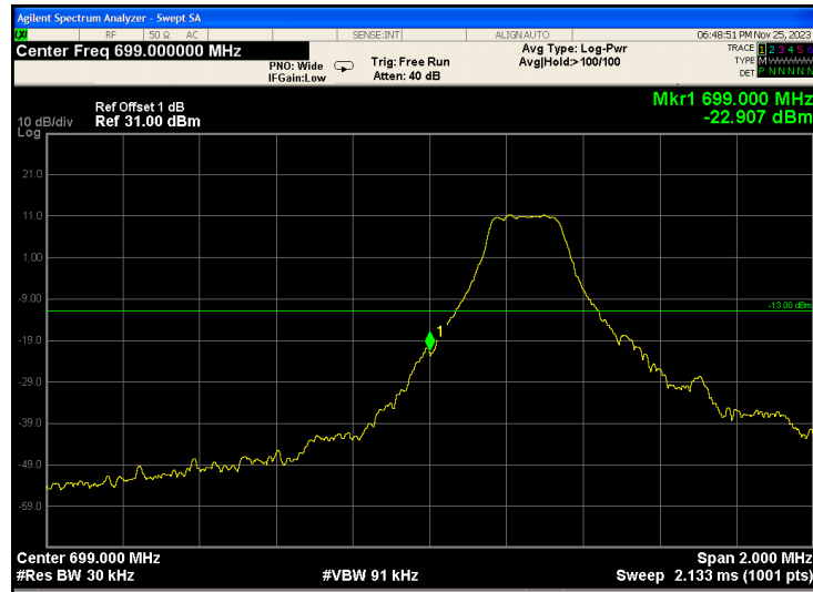
Band12-1.4MHz-QPSK-23017-1RB#5
