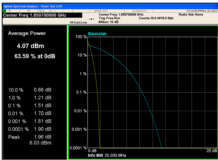
Band2-1.4MHz-QPSK-18607-6RB#0
