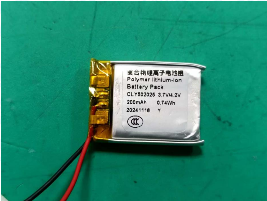
Photo 10 Battery Appearance
