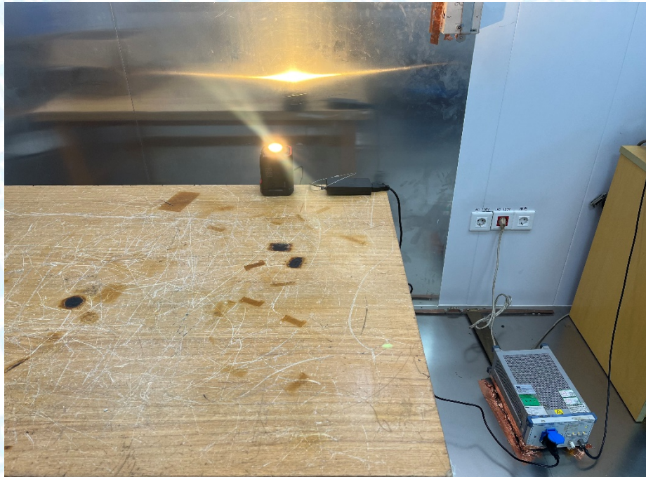
Photo of Setup for Radiated Emission (30MHz~1GHz)
